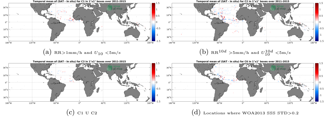
Figure 11: Temporal mean gridded over spatial boxes of size 1^\circ \times 1^\circ of \Delta SSS (Aquarius-L4-IPRC-V5-WEEKLY - Surface drifters) for 4 different subdatasets corresponding to: RR > 1\text{mm/h} and U_{10} < 5\text{m/s} (a), RR^{10d} > 5\text{mm/h} and U_{10}^{10d} < 5\text{m/s} (b), C1 U C2 (c), Locations where WOA2013 SSS STD > 0.2 (d).
