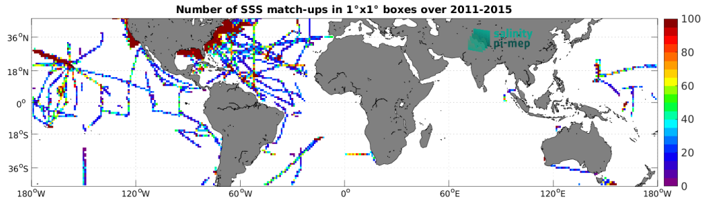
Figure 5: Number of SSS match-ups between TSG (SAMOS) SSS and the Aquarius SSS L4 OI v5 - Monthly (IPRC) SSS product for the Mid-Low Latitudes 45N-45S Pi-MEP region over 1^\circ \times 1^\circ boxes and for the full satellite product period.
