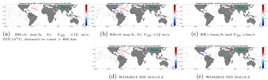
Figure 14: Temporal mean gridded over spatial boxes of size 1^\circ \times 1^\circ of \Delta\text{SSS} (Aquarius SSS L4 OI v5 - Monthly (IPRC) - TSG (SAMOS)) for 5 different subdatasets corresponding to: RR=0 mm/h, 3 < U_{10} < 12 m/s, SST > 5°C, distance to coast > 800 km (a), RR=0 mm/h, 3 < U_{10} < 12 m/s (b), RR > 1mm/h and U_{10} < 4 m/s (c), WOA2013 SSS Std < 0.2 (d), WOA2013 SSS Std > 0.2 (e).
