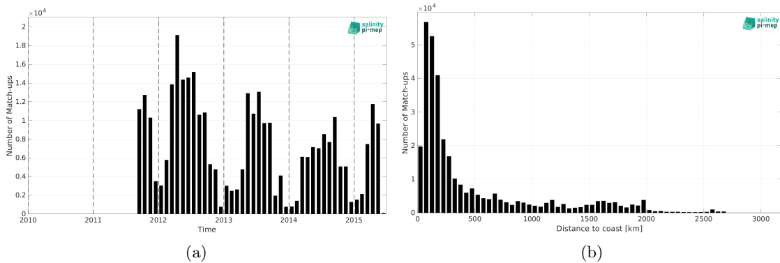
Figure 2: Number of match-ups between TSG (SAMOS) and Aquarius SSS L4 OI v5 - Monthly (IPRC) SSS as a function of time (a) and as function of the distance to coast (b) over the Mid-Low Latitudes 45N-45S Pi-MEP region and for the full satellite product period.
