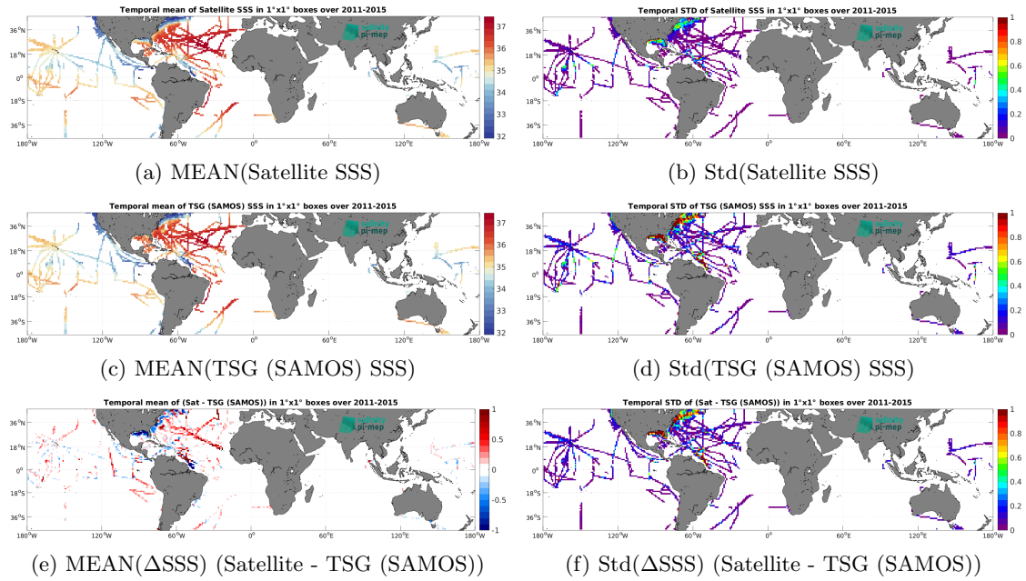
Figure 7: Temporal mean (left) and Std (right) of SSS from Aquarius SSS L4 OI v5 - Monthly (IPRC) (top), TSG (SAMOS) (middle), and of \Delta SSS (Satellite - TSG (SAMOS)). Only match-up pairs are used to generate these maps.
