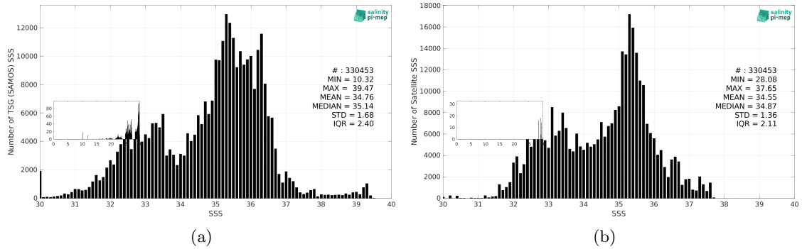
Figure 3: Histograms of SSS from TSG (SAMOS) (a) and Aquarius SSS L4 OI v5 - Monthly (IPRC) (b) considering all match-up pairs per bins of 0.1 over the Mid-Low Latitudes 45N-45S Pi-MEP region and for the full satellite product period.
