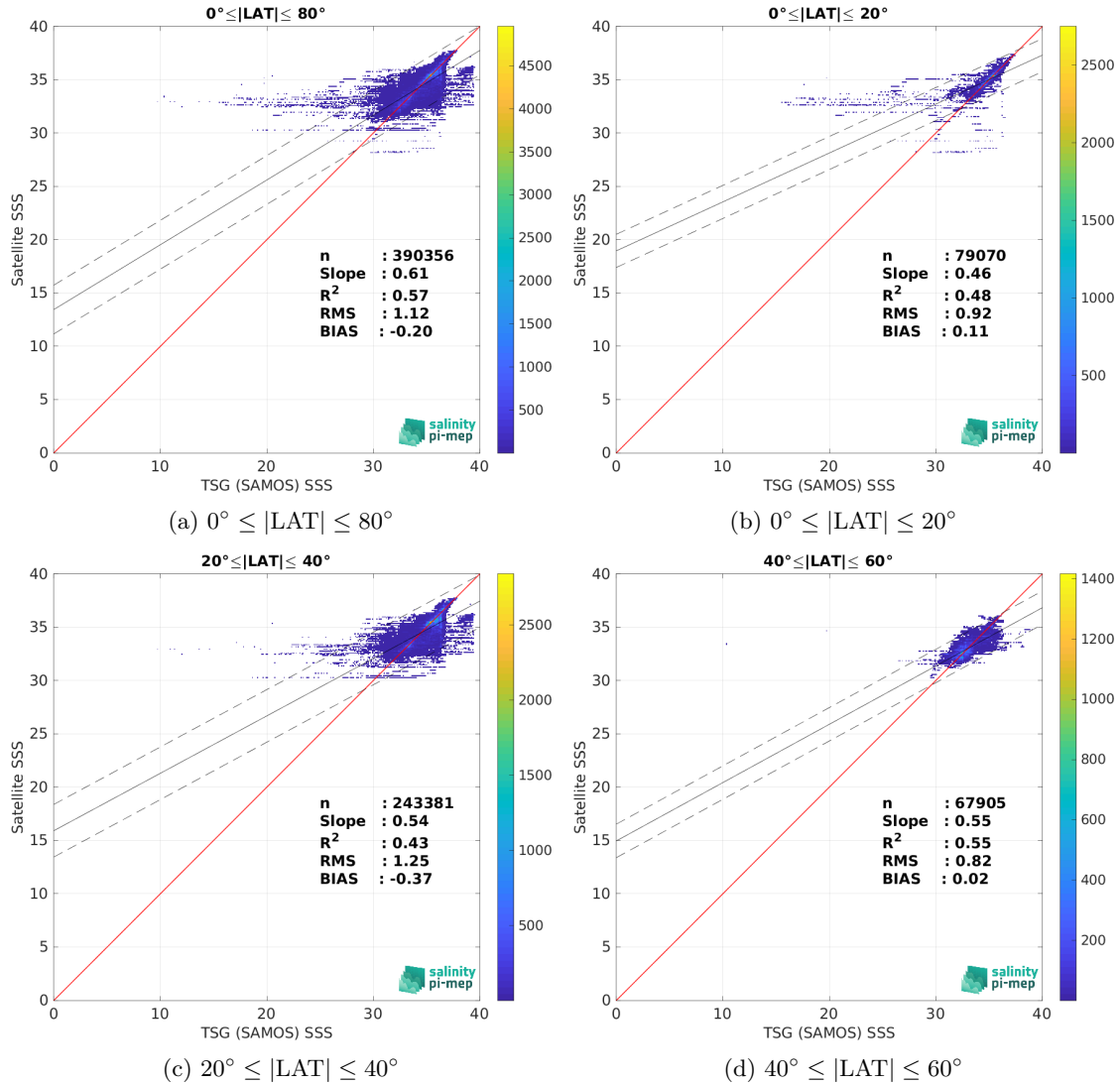
Figure 9: Contour maps of the concentration of Aquarius SSS L4 OI v5 - Monthly (IPRC) SSS (y-axis) versus TSG (SAMOS) SSS (x-axis) at match-up pairs for different latitude bands. For each plot, the red line shows x=y . The black thin and dashed lines indicate a linear fit through the data cloud and the \pm 95\% confidence levels, respectively. The number match-up pairs n , the slope and R^2 coefficient of the linear fit, the root mean square (RMS) and the mean bias between satellite and in situ data are indicated for each latitude band in each plot.
