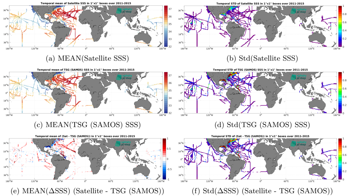
Figure 6: Temporal mean (left) and Std (right) of SSS from Aquarius SSS L4 OI v5 - Monthly (IPRC) (top), TSG (SAMOS) (middle), and of \Delta SSS (Satellite - TSG (SAMOS)). Only match-up pairs are used to generate these maps.
