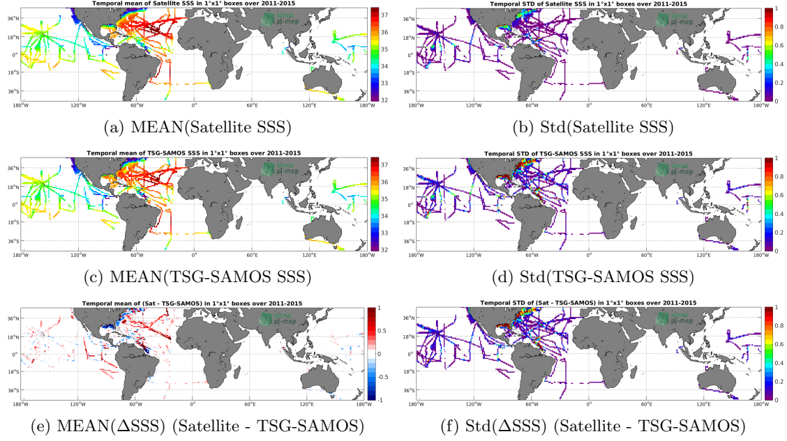
Figure 6: Temporal mean (left) and Std (right) of SSS from Aquarius-L4-IPRC-V5-MONTHLY (top), TSG-SAMOS (middle), and of \Delta SSS (Satellite - TSG-SAMOS). Only match-up pairs are used to generate these maps.
