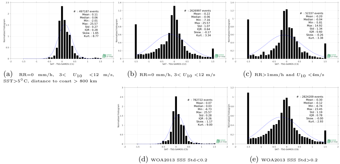
Figure 13: Normalized histogram of \Delta SSS (Aquarius-L4-IPRC-V5-MONTHLY - TSG-SAMOS) for 5 different subdatasets corresponding to: RR=0 mm/h, 3 < U_{10} < 12 m/s, SST >5^\circ\text{C} , distance to coast > 800 km (a), RR=0 mm/h, 3 < U_{10} < 12 m/s (b), RR >1 mm/h and U_{10} < 4 m/s (c), WOA2013 SSS Std <0.2 (d), WOA2013 SSS Std >0.2 (e).
