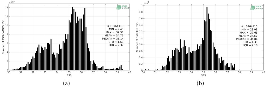
Figure 2: Histograms of SSS from TSG-SAMOS (a) and Aquarius-L4-IPRC-V5-MONTHLY (b) considering all match-up pairs per bins of 0.1 over the Mid-Low Latitudes 45N-45S Pi-MEP region and for the full satellite product period.
