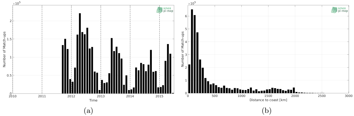
Figure 1: Number of match-ups between TSG-SAMOS and Aquarius-L4-IPRC-V5-MONTHLY SSS as a function of time (a) and as function of the distance to coast (b) over the Mid-Low Latitudes 45N-45S Pi-MEP region and for the full satellite product period.
