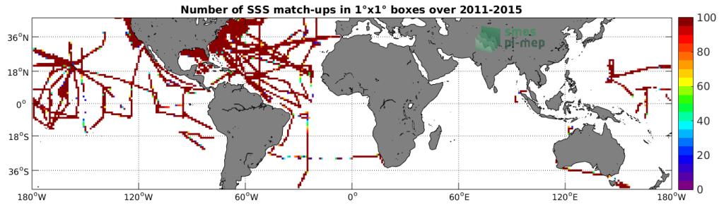
Figure 4: Number of SSS match-ups between TSG-SAMOS SSS and the Aquarius-L4-IPRC-V5-MONTHLY SSS product for the Mid-Low Latitudes 45N-45S Pi-MEP region over 1°x1° boxes and for the full satellite product period.
