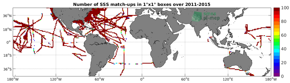
Figure 4: Number of SSS match-ups between TSG-SAMOS SSS and the Aquarius-L4-IPRC-V5-MONTHLY SSS product for the Mid-Low Latitudes 45N-45S Pi-MEP region over 1^\circ \times 1^\circ boxes and for the full satellite product period.
