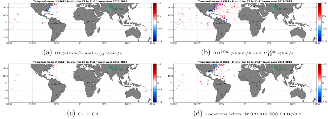
Figure 12: Temporal mean gridded over spatial boxes of size 1^\circ \times 1^\circ of \Delta SSS (Aquarius-L4-IPRC-V5-MONTHLY - TSG-SAMOS) for 4 different subdatasets corresponding to: RR > 1mm/h and U_{10} < 5\text{m/s} (a), RR^{10d} > 5\text{mm/h} and U_{10}^{10d} < 5\text{m/s} (b), C1 U C2 (c), Locations where WOA2013 SSS STD > 0.2 (d).
