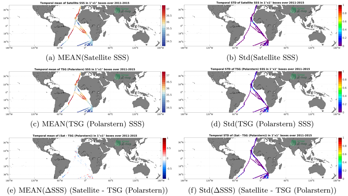
Figure 6: Temporal mean (left) and Std (right) of SSS from Aquarius SSS L4 OI v5 - Monthly (IPRC) (top), TSG (Polarstern) (middle), and of \Delta SSS (Satellite - TSG (Polarstern)). Only match-up pairs are used to generate these maps.
