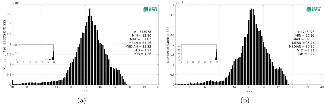
Figure 3: Histograms of SSS from TSG (LEGOS-DM) (a) and Aquarius SSS L4 OI v5 - Monthly (IPRC) (b) considering all match-up pairs per bins of 0.1 over the Mid-Low Latitudes 45N-45S Pi-MEP region and for the full satellite product period.
