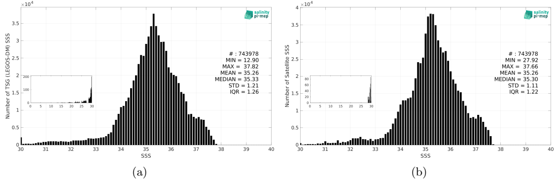
Figure 3: Histograms of SSS from TSG (LEGOS-DM) (a) and Aquarius SSS L4 OI v5 - Monthly (IPRC) (b) considering all match-up pairs per bins of 0.1 over the Mid-Low Latitudes 45N-45S Pi-MEP region and for the full satellite product period.
