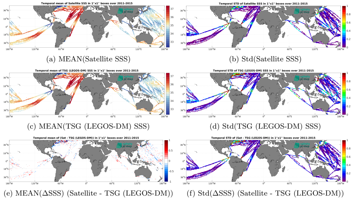
Figure 7: Temporal mean (left) and Std (right) of SSS from Aquarius SSS L4 OI v5 - Monthly (IPRC) (top), TSG (LEGOS-DM) (middle), and of \Delta SSS (Satellite - TSG (LEGOS-DM)). Only match-up pairs are used to generate these maps.
