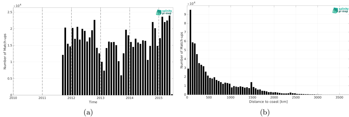
Figure 2: Number of match-ups between TSG (LEGOS-DM) and Aquarius SSS L4 OI v5 - Monthly (IPRC) SSS as a function of time (a) and as function of the distance to coast (b) over the Mid-Low Latitudes 45N-45S Pi-MEP region and for the full satellite product period.
