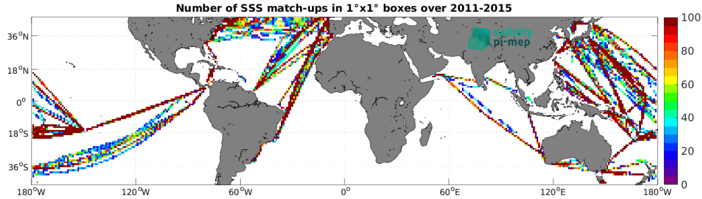
Figure 5: Number of SSS match-ups between TSG (LEGOS-DM) SSS and the Aquarius SSS L4 OI v5 - Monthly (IPRC) SSS product for the Mid-Low Latitudes 45N-45S Pi-MEP region over 1^\circ \times 1^\circ boxes and for the full satellite product period.
