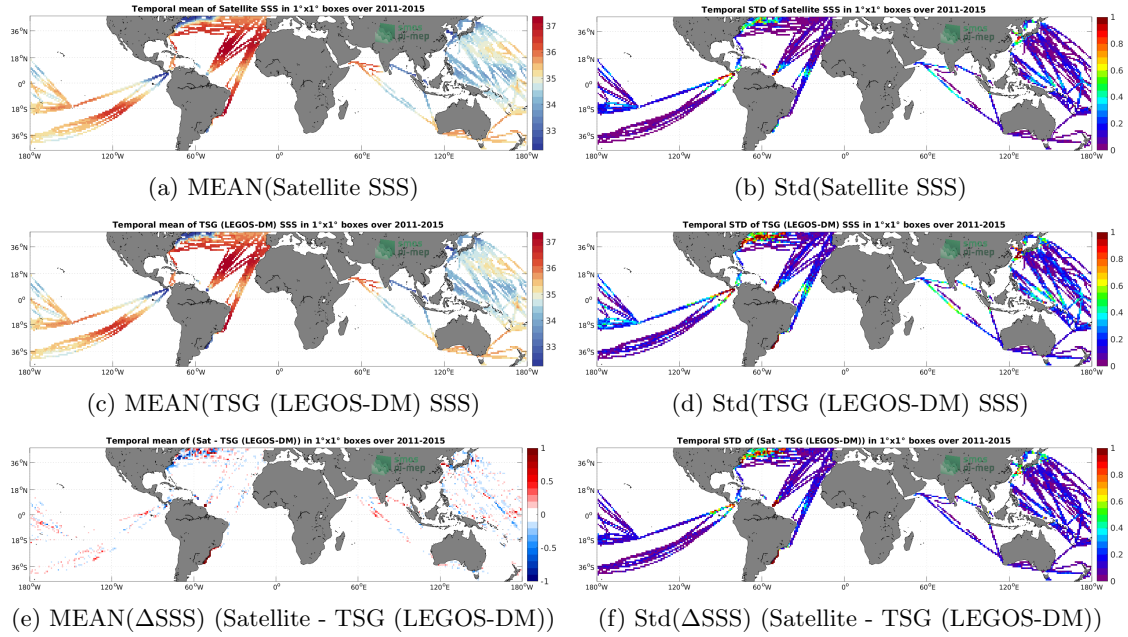
Figure 6: Temporal mean (left) and Std (right) of SSS from Aquarius SSS L4 OI v5 - Monthly (IPRC) (top), TSG (LEGOS-DM) (middle), and of \Delta SSS (Satellite - TSG (LEGOS-DM)). Only match-up pairs are used to generate these maps.
