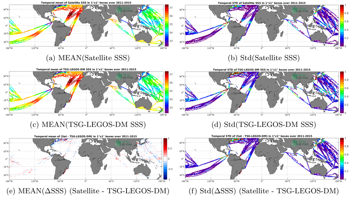
Figure 6: Temporal mean (left) and Std (right) of SSS from Aquarius-L4-IPRC-V5-MONTHLY (top), TSG-LEGOS-DM (middle), and of \Delta SSS (Satellite - TSG-LEGOS-DM). Only match-up pairs are used to generate these maps.
