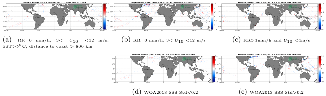
Figure 12: Temporal mean gridded over spatial boxes of size 1°x1° of \Delta SSS (Aquarius-L4-IPRC-V5-MONTHLY - TSG-LEGOS-DM) for 5 different subdatasets corresponding to:RR=0 mm/h, 3 < U_{10} < 12 m/s, SST>5°C, distance to coast > 800 km (a), RR=0 mm/h, 3 < U_{10} < 12 m/s (b), RR>1mm/h and U_{10} < 4m/s (c), WOA2013 SSS Std<0.2 (d), WOA2013 SSS Std>0.2 (e).
