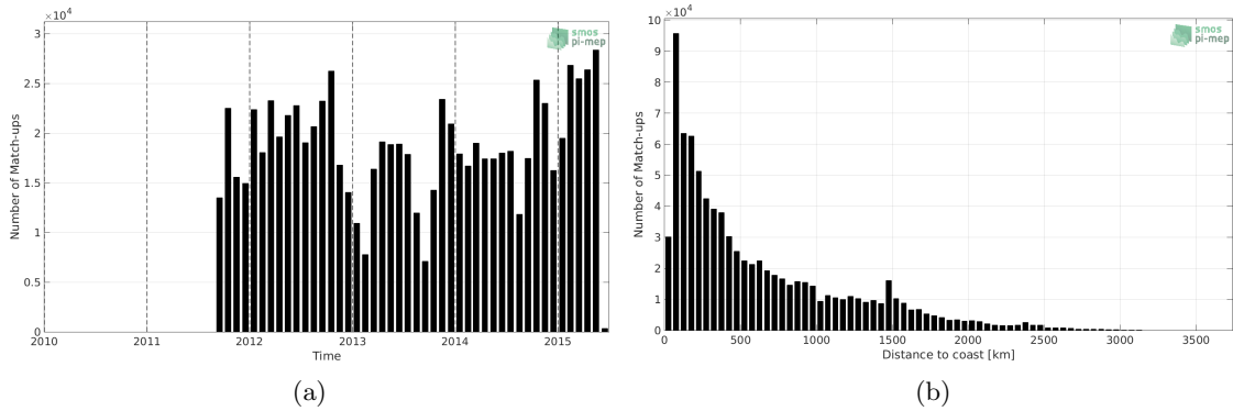
Figure 1: Number of match-ups between TSG-LEGOS-DM and Aquarius-L4-IPRC-V5-MONTHLY SSS as a function of time (a) and as function of the distance to coast (b) over the Mid-Low Latitudes 45N-45S Pi-MEP region and for the full satellite product period.
