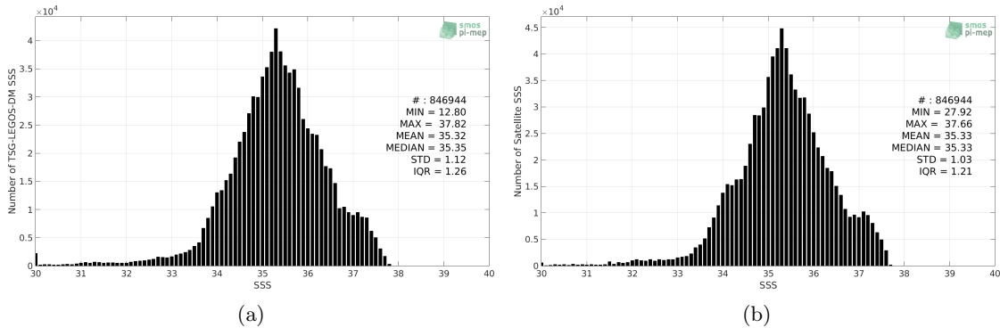
Figure 2: Histograms of SSS from TSG-LEGOS-DM (a) and Aquarius-L4-IPRC-V5-MONTHLY (b) considering all match-up pairs per bins of 0.1 over the Mid-Low Latitudes 45N-45S Pi-MEP region and for the full satellite product period.
