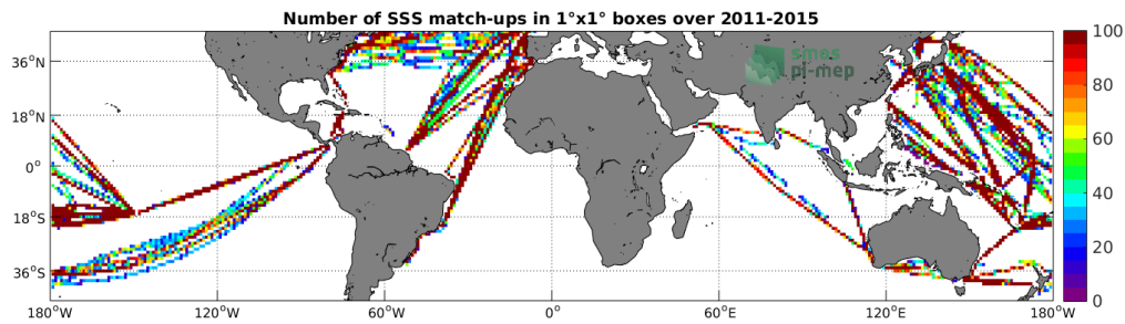
Figure 4: Number of SSS match-ups between TSG-LEGOS-DM SSS and the Aquarius-L4-IPRC-V5-MONTHLY SSS product for the Mid-Low Latitudes 45N-45S Pi-MEP region over 1^\circ \times 1^\circ boxes and for the full satellite product period.
