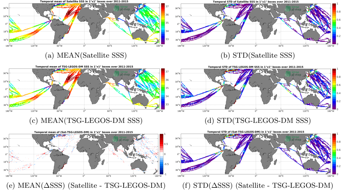
Figure 6: Temporal mean (left) and STD (right) of SSS from Aquarius-L4-IPRC-V5-MONTHLY (top), TSG-LEGOS-DM (middle), and of \Delta SSS (Satellite - TSG-LEGOS-DM). Only match-up pairs are used to generate these maps.
