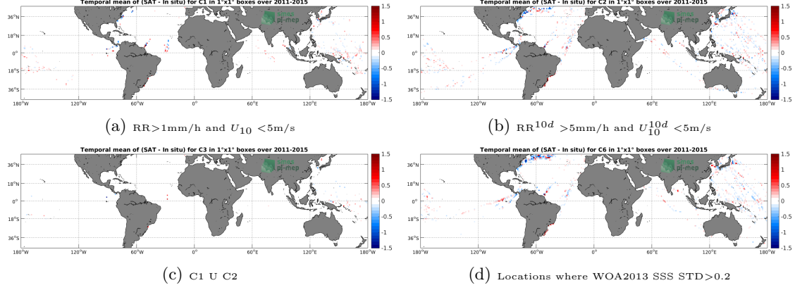
Figure 12: Temporal mean gridded over spatial boxes of size 1^\circ \times 1^\circ of \Delta SSS (Aquarius-L4-IPRC-V5-MONTHLY - TSG-LEGOS-DM) for 4 different subdatasets corresponding to: RR > 1\text{mm/h} and U_{10} < 5\text{m/s} (a), RR^{10d} > 5\text{mm/h} and U_{10}^{10d} < 5\text{m/s} (b), C1 U C2 (c), Locations where WOA2013 SSS STD > 0.2 (d).
