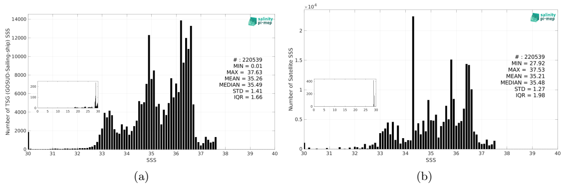
Figure 3: Histograms of SSS from TSG (GOSUD-Sailing-ship) (a) and Aquarius SSS L4 OI v5 - Monthly (IPRC) (b) considering all match-up pairs per bins of 0.1 over the Mid-Low Latitudes 45N-45S Pi-MEP region and for the full satellite product period.
