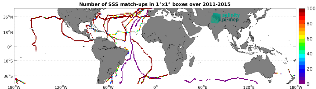
Figure 5: Number of SSS match-ups between TSG (GOSUD-Sailing-ship) SSS and the Aquarius SSS L4 OI v5 - Monthly (IPRC) SSS product for the Mid-Low Latitudes 45N-45S Pi-MEP region over 1^\circ \times 1^\circ boxes and for the full satellite product period.
