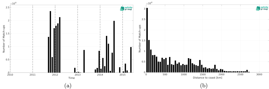
Figure 2: Number of match-ups between TSG (GOSUD-Sailing-ship) and Aquarius SSS L4 OI v5 - Monthly (IPRC) SSS as a function of time (a) and as function of the distance to coast (b) over the Mid-Low Latitudes 45N-45S Pi-MEP region and for the full satellite product period.
