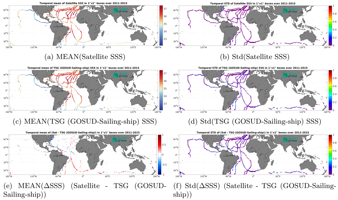
Figure 7: Temporal mean (left) and Std (right) of SSS from Aquarius SSS L4 OI v5 - Monthly (IPRC) (top), TSG (GOSUD-Sailing-ship) (middle), and of \Delta SSS (Satellite - TSG (GOSUD-Sailing-ship)). Only match-up pairs are used to generate these maps.
