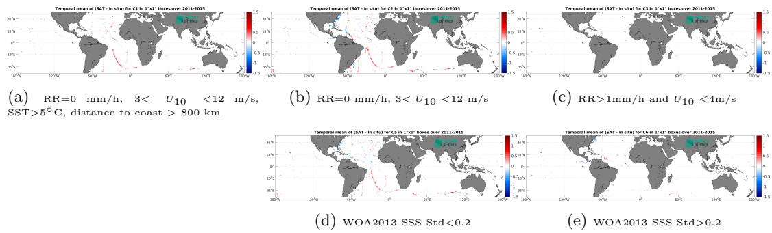
Figure 14: Temporal mean gridded over spatial boxes of size 1^\circ \times 1^\circ of \Delta\text{SSS} (Aquarius SSS L4 OI v5 - Monthly (IPRC) - TSG (GOSUD-Sailing-ship)) for 5 different subdatasets corresponding to:RR=0 mm/h, 3 < U_{10} < 12 m/s, SST>5°C, distance to coast > 800 km (a), RR=0 mm/h, 3 < U_{10} < 12 m/s (b), RR>1mm/h and U_{10} < 4 m/s (c), WOA2013 SSS Std<0.2 (d), WOA2013 SSS Std>0.2 (e).
