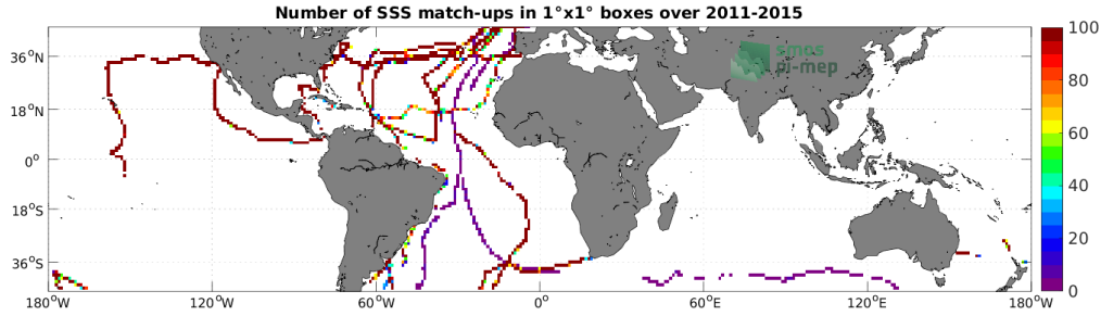
Figure 4: Number of SSS match-ups between TSG (GOSUD-Sailing-ship) SSS and the Aquarius SSS L4 OI v5 - Monthly (IPRC) SSS product for the Mid-Low Latitudes 45N-45S Pi-MEP region over 1^\circ \times 1^\circ boxes and for the full satellite product period.
