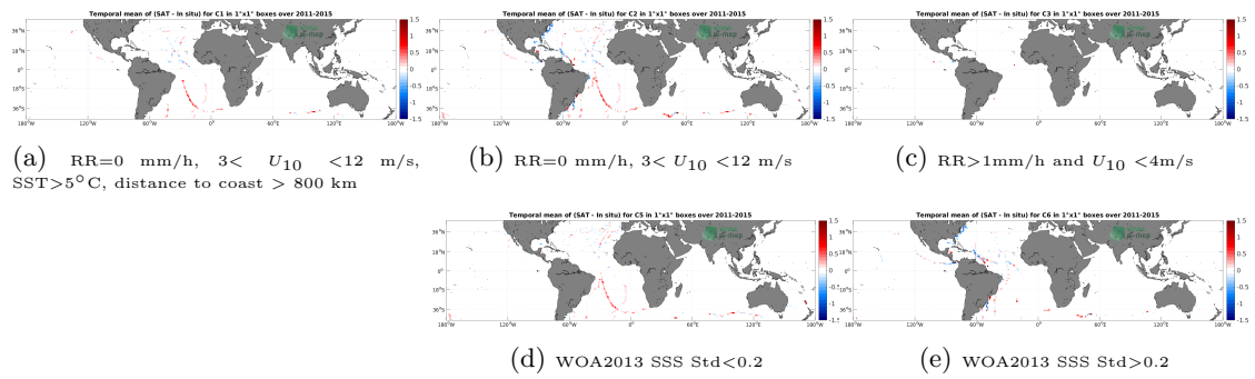
Figure 12: Temporal mean gridded over spatial boxes of size 1^\circ \times 1^\circ of \Delta SSS (Aquarius SSS L4 OI v5 - Monthly (IPRC) - TSG (GOSUD-Sailing-ship)) for 5 different subdatasets corresponding to:RR=0 mm/h, 3 < U_{10} < 12 m/s, SST>5°C, distance to coast > 800 km (a), RR=0 mm/h, 3 < U_{10} < 12 m/s (b), RR>1mm/h and U_{10} < 4 m/s (c), WOA2013 SSS Std<0.2 (d), WOA2013 SSS Std>0.2 (e).
