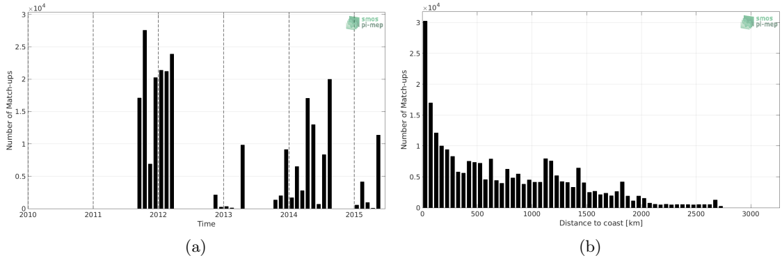
Figure 1: Number of match-ups between TSG-GOSUD-Sailing-ship and Aquarius-L4-IPRC-V5-MONTHLY SSS as a function of time (a) and as function of the distance to coast (b) over the Mid-Low Latitudes 45N-45S Pi-MEP region and for the full satellite product period.
