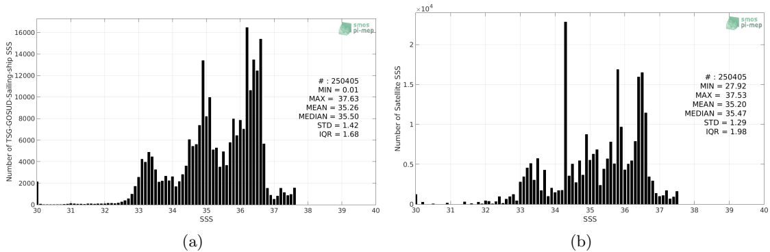
Figure 2: Histograms of SSS from TSG-GOSUD-Sailing-ship (a) and Aquarius-L4-IPRC-V5-MONTHLY (b) considering all match-up pairs per bins of 0.1 over the Mid-Low Latitudes 45N-45S Pi-MEP region and for the full satellite product period.
