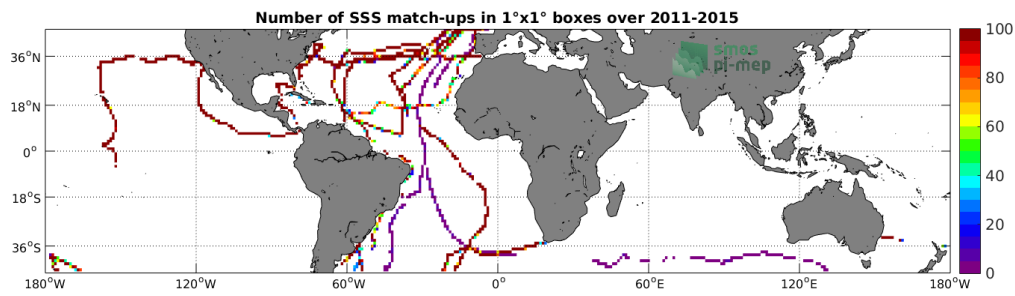
Figure 4: Number of SSS match-ups between TSG-GOSUD-Sailing-ship SSS and the Aquarius-L4-IPRC-V5-MONTHLY SSS product for the Mid-Low Latitudes 45N-45S Pi-MEP region over 1°x1° boxes and for the full satellite product period.
