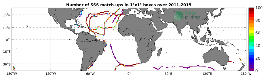
Figure 4: Number of SSS match-ups between TSG-GOSUD-Sailing-ship SSS and the Aquarius-L4-IPRC-V5-MONTHLY SSS product for the Mid-Low Latitudes 45N-45S Pi-MEP region over 1^\circ \times 1^\circ boxes and for the full satellite product period.
