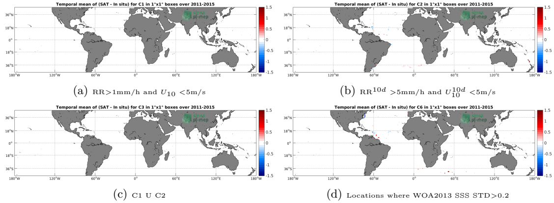
Figure 12: Temporal mean gridded over spatial boxes of size 1^\circ \times 1^\circ of \Delta SSS (Aquarius-L4-IPRC-V5-MONTHLY - TSG-GOSUD-Sailing-ship) for 4 different subdatasets corresponding to: RR > 1\text{mm/h} and U_{10} < 5\text{m/s} (a), RR^{10d} > 5\text{mm/h} and U_{10}^{10d} < 5\text{m/s} (b), C1 U C2 (c), Locations where WOA2013 SSS STD > 0.2 (d).
