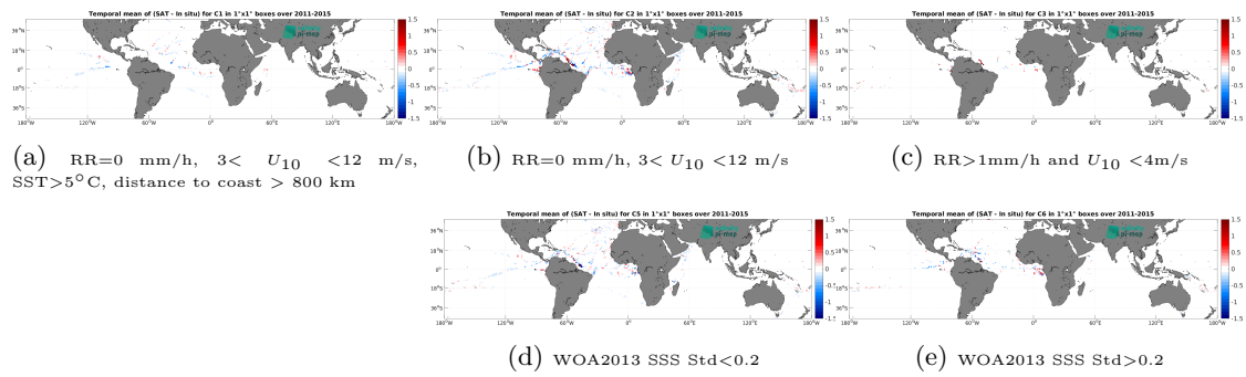
Figure 12: Temporal mean gridded over spatial boxes of size 1^\circ \times 1^\circ of \Delta\text{SSS} (Aquarius SSS L4 OI v5 - Monthly (IPRC) - TSG (GOSUD-Research-vessel)) for 5 different subdatasets corresponding to: RR=0 mm/h, 3 < U_{10} < 12 m/s, SST > 5°C, distance to coast > 800 km (a), RR=0 mm/h, 3 < U_{10} < 12 m/s (b), RR > 1mm/h and U_{10} < 4 m/s (c), WOA2013 SSS Std < 0.2 (d), WOA2013 SSS Std > 0.2 (e).
