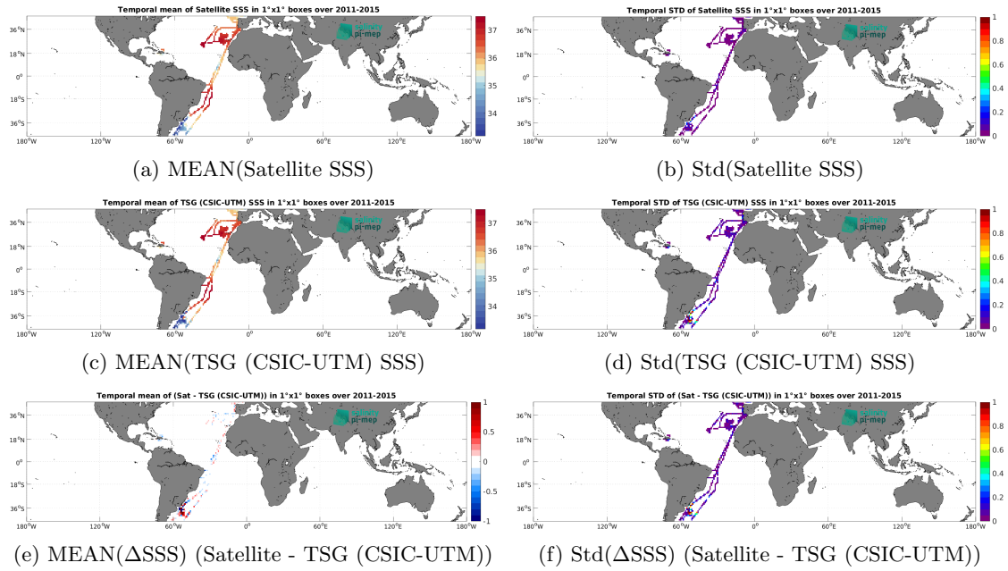
Figure 7: Temporal mean (left) and Std (right) of SSS from Aquarius SSS L4 OI v5 - Monthly (IPRC) (top), TSG (CSIC-UTM) (middle), and of \Delta SSS (Satellite - TSG (CSIC-UTM)). Only match-up pairs are used to generate these maps.
