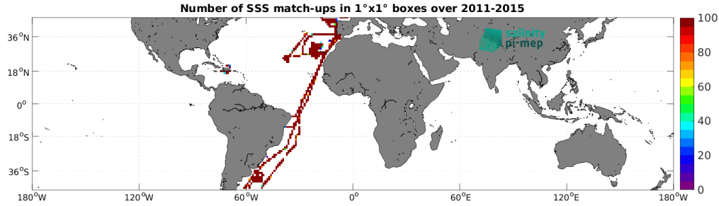
Figure 5: Number of SSS match-ups between TSG (CSIC-UTM) SSS and the Aquarius SSS L4 OI v5 - Monthly (IPRC) SSS product for the Mid-Low Latitudes 45N-45S Pi-MEP region over 1^\circ \times 1^\circ boxes and for the full satellite product period.
