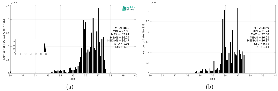
Figure 3: Histograms of SSS from TSG (CSIC-UTM) (a) and Aquarius SSS L4 OI v5 - Monthly (IPRC) (b) considering all match-up pairs per bins of 0.1 over the Mid-Low Latitudes 45N-45S Pi-MEP region and for the full satellite product period.
