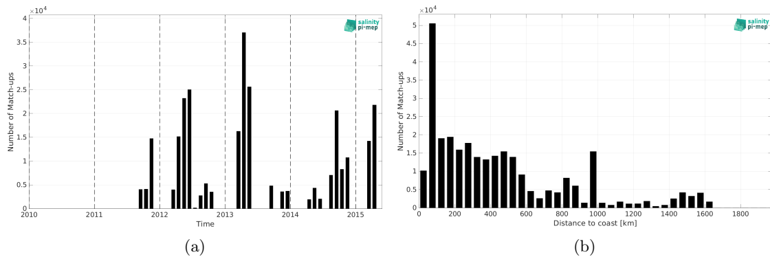
Figure 2: Number of match-ups between TSG (CSIC-UTM) and Aquarius SSS L4 OI v5 - Monthly (IPRC) SSS as a function of time (a) and as function of the distance to coast (b) over the Mid-Low Latitudes 45N-45S Pi-MEP region and for the full satellite product period.
