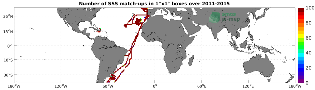
Figure 4: Number of SSS match-ups between TSG (CSIC-UTM) SSS and the Aquarius SSS L4 OI v5 - Monthly (IPRC) SSS product for the Mid-Low Latitudes 45N-45S Pi-MEP region over 1^\circ \times 1^\circ boxes and for the full satellite product period.
