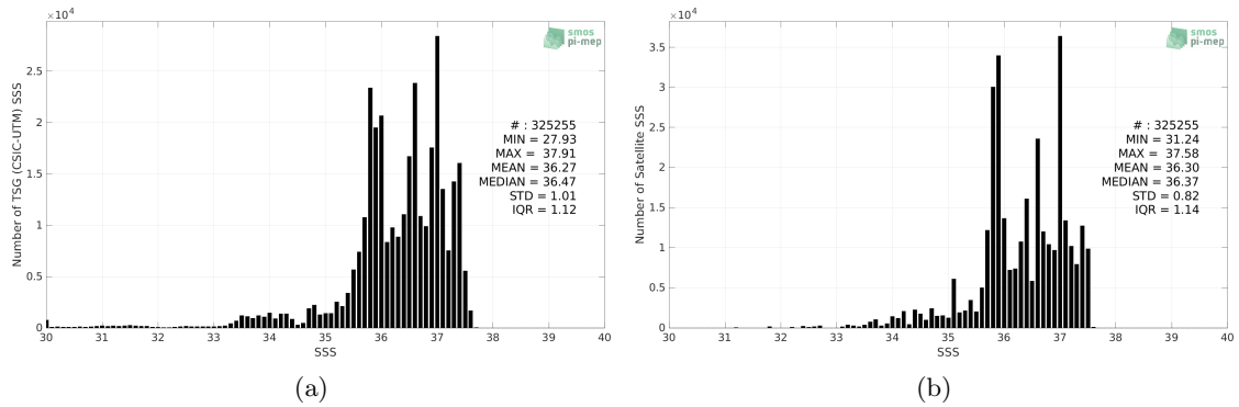
Figure 2: Histograms of SSS from TSG (CSIC-UTM) (a) and Aquarius SSS L4 OI v5 - Monthly (IPRC) (b) considering all match-up pairs per bins of 0.1 over the Mid-Low Latitudes 45N-45S Pi-MEP region and for the full satellite product period.
