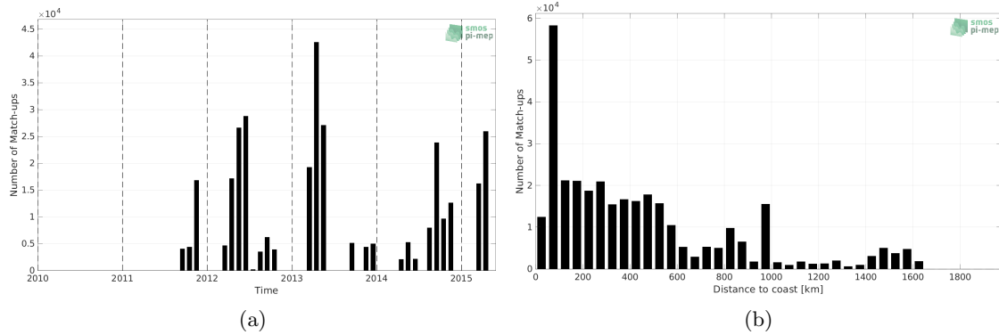
Figure 1: Number of match-ups between TSG (CSIC-UTM) and Aquarius SSS L4 OI v5 - Monthly (IPRC) SSS as a function of time (a) and as function of the distance to coast (b) over the Mid-Low Latitudes 45N-45S Pi-MEP region and for the full satellite product period.
