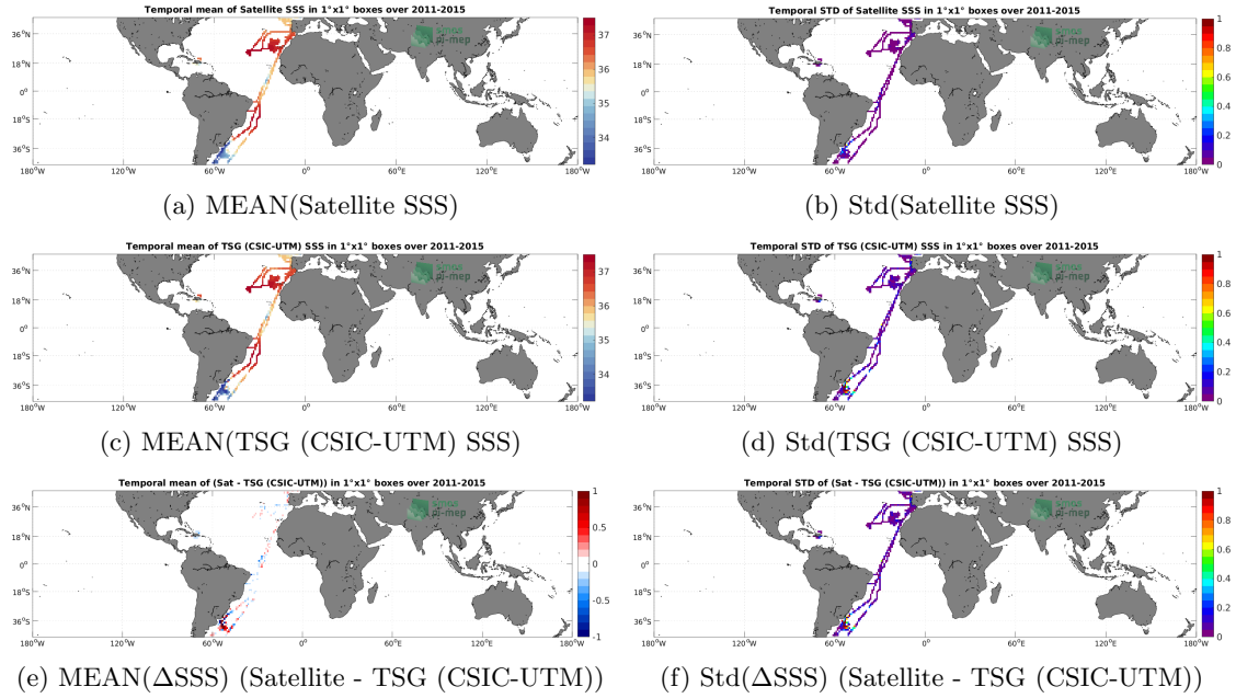
Figure 6: Temporal mean (left) and Std (right) of SSS from Aquarius SSS L4 OI v5 - Monthly (IPRC) (top), TSG (CSIC-UTM) (middle), and of \Delta SSS (Satellite - TSG (CSIC-UTM)). Only match-up pairs are used to generate these maps.
