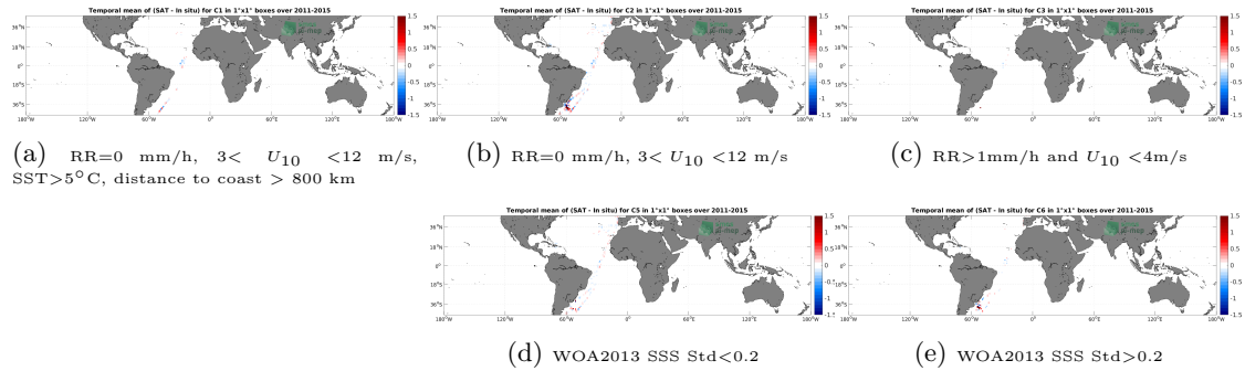
Figure 12: Temporal mean gridded over spatial boxes of size 1^\circ \times 1^\circ of \Delta\text{SSS} (Aquarius SSS L4 OI v5 - Monthly (IPRC) - TSG (CSIC-UTM)) for 5 different subdatasets corresponding to:RR=0 mm/h, 3 < U_{10} < 12 m/s, SST >5^\circ\text{C} , distance to coast > 800 km (a), RR=0 mm/h, 3 < U_{10} < 12 m/s (b), RR >1 mm/h and U_{10} < 4 m/s (c), WOA2013 SSS Std <0.2 (d), WOA2013 SSS Std >0.2 (e).
