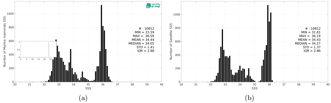
Figure 3: Histograms of SSS from Marine mammals (a) and Aquarius SSS L4 OI v5 - Monthly (IPRC) (b) considering all match-up pairs per bins of 0.1 over the Mid-Low Latitudes 45N-45S Pi-MEP region and for the full satellite product period.
