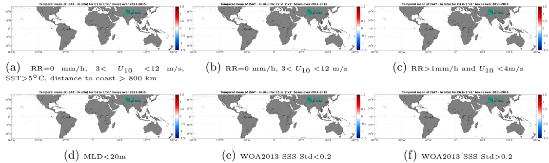
Figure 14: Temporal mean gridded over spatial boxes of size 1^\circ \times 1^\circ of \Delta SSS (Aquarius SSS L4 OI v5 - Monthly (IPRC) - Marine mammals) for 6 different subdatasets corresponding to:RR=0 mm/h, 3 < U_{10} < 12 m/s, SST>5°C, distance to coast > 800 km (a), RR=0 mm/h, 3 < U_{10} < 12 m/s (b), RR>1mm/h and U_{10} < 4 m/s (c),MLD<20m (d),WOA2013 SSS Std<0.2 (e),WOA2013 SSS Std>0.2 (f).
