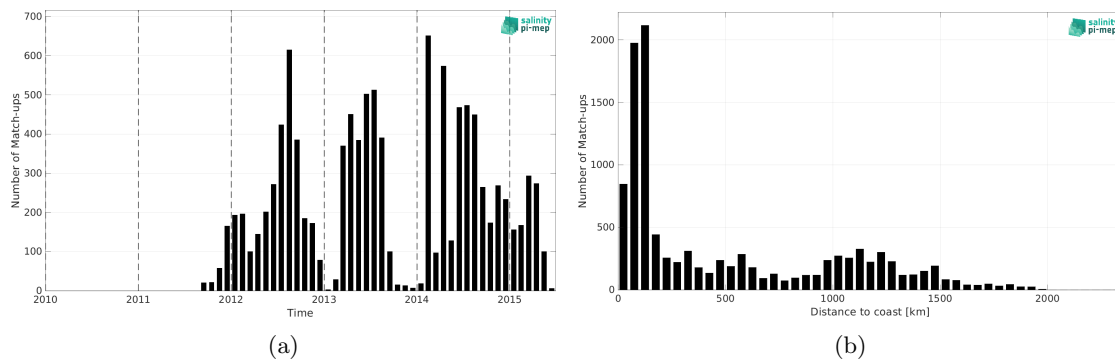
Figure 2: Number of match-ups between Marine mammals and Aquarius SSS L4 OI v5 - Monthly (IPRC) SSS as a function of time (a) and as function of the distance to coast (b) over the Mid-Low Latitudes 45N-45S Pi-MEP region and for the full satellite product period.
