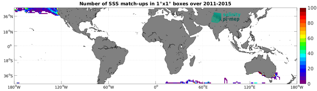
Figure 5: Number of SSS match-ups between Marine mammals SSS and the Aquarius SSS L4 OI v5 - Monthly (IPRC) SSS product for the Mid-Low Latitudes 45N-45S Pi-MEP region over 1^\circ \times 1^\circ boxes and for the full satellite product period.
