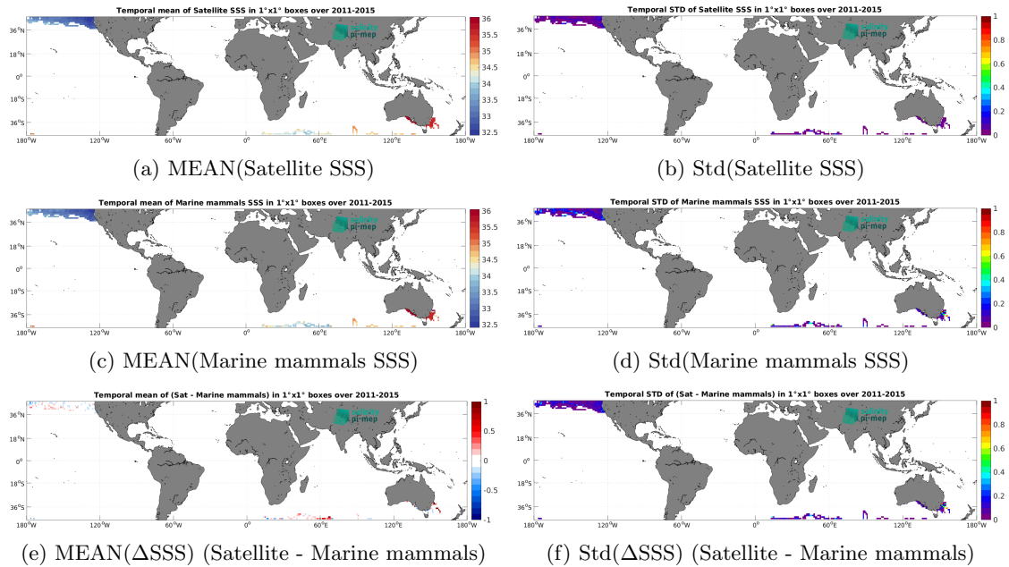
Figure 7: Temporal mean (left) and Std (right) of SSS from Aquarius SSS L4 OI v5 - Monthly (IPRC) (top), Marine mammals (middle), and of \Delta SSS (Satellite - Marine mammals). Only match-up pairs are used to generate these maps.
