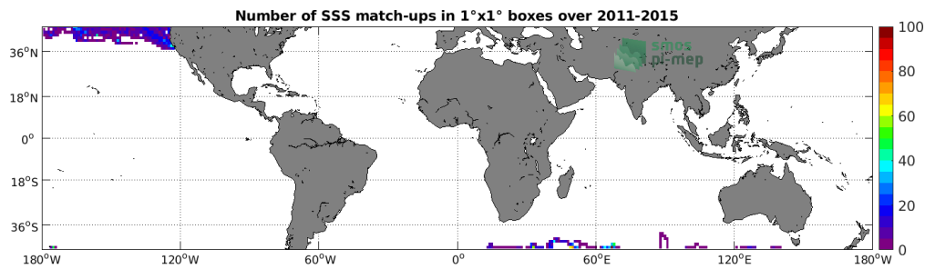
Figure 4: Number of SSS match-ups between Sea mammals SSS and the Aquarius SSS L4 OI v5 - Monthly (IPRC) SSS product for the Mid-Low Latitudes 45N-45S Pi-MEP region over 1^\circ \times 1^\circ boxes and for the full satellite product period.
