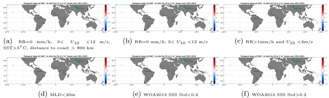
Figure 12: Temporal mean gridded over spatial boxes of size 1°x1° of \Delta SSS (Aquarius SSS L4 OI v5 - Monthly (IPRC) - Sea mammals) for 6 different subdatasets corresponding to:RR=0 mm/h, 3 < U_{10} < 12 m/s, SST > 5^{\circ}C , distance to coast > 800 km (a), RR=0 mm/h, 3 < U_{10} < 12 m/s (b), RR>1mm/h and U_{10} < 4m/s (c),MLD<20m (d),WOA2013 SSS Std<0.2 (e),WOA2013 SSS Std>0.2 (f).
