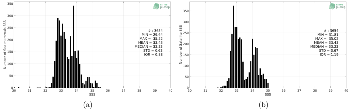
Figure 2: Histograms of SSS from Sea mammals (a) and Aquarius SSS L4 OI v5 - Monthly (IPRC) (b) considering all match-up pairs per bins of 0.1 over the Mid-Low Latitudes 45N-45S Pi-MEP region and for the full satellite product period.
