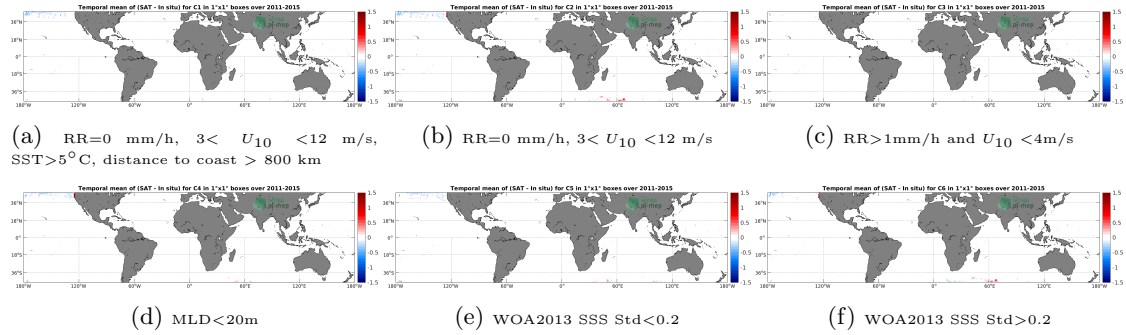
Figure 12: Temporal mean gridded over spatial boxes of size 1^\circ \times 1^\circ of \Delta SSS (Aquarius SSS L4 OI v5 - Monthly (IPRC) - Sea mammals) for 6 different subdatasets corresponding to: RR=0 mm/h, 3 < U_{10} < 12 m/s, SST > 5^\circ C , distance to coast > 800 km (a), RR=0 mm/h, 3 < U_{10} < 12 m/s (b), RR > 1 mm/h and U_{10} < 4 m/s (c), MLD < 20 m (d), WOA2013 SSS Std < 0.2 (e), WOA2013 SSS Std > 0.2 (f).
