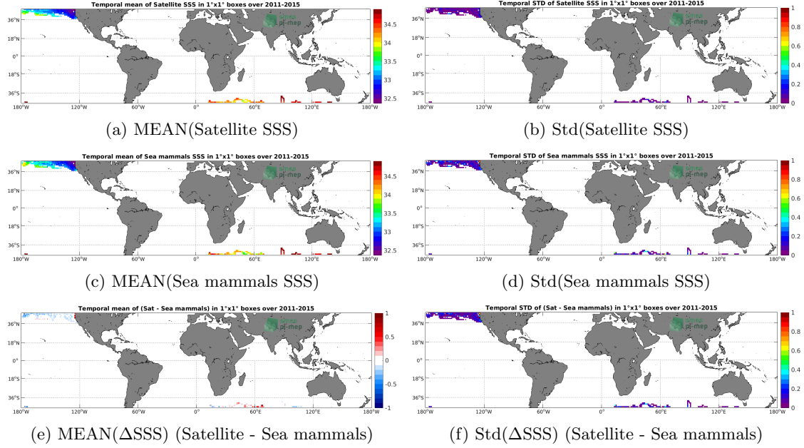
Figure 6: Temporal mean (left) and Std (right) of SSS from Aquarius SSS L4 OI v5 - Monthly (IPRC) (top), Sea mammals (middle), and of \Delta SSS (Satellite - Sea mammals). Only match-up pairs are used to generate these maps.
