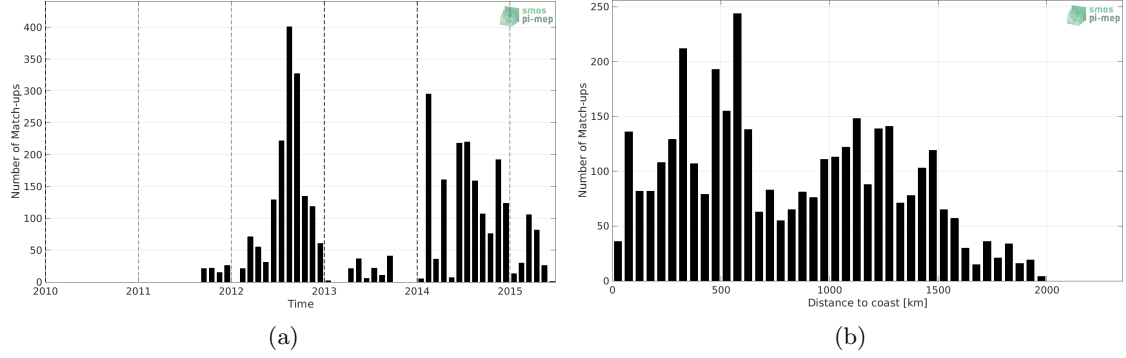
Figure 1: Number of match-ups between Sea mammals and Aquarius SSS L4 OI v5 - Monthly (IPRC) SSS as a function of time (a) and as function of the distance to coast (b) over the Mid-Low Latitudes 45N-45S Pi-MEP region and for the full satellite product period.
