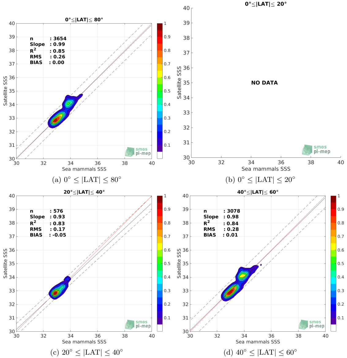
Figure 9: Contour maps of the concentration of Aquarius SSS L4 OI v5 - Monthly (IPRC) SSS (y-axis) versus Sea mammals SSS (x-axis) at match-up pairs for different latitude bands. For each plot, the red line shows x=y . The black thin and dashed lines indicate a linear fit through the data cloud and the \pm 95\% confidence levels, respectively. The number match-up pairs n , the slope and R^2 coefficient of the linear fit, the root mean square (RMS) and the mean bias between satellite and in situ data are indicated for each latitude band in each plots.
