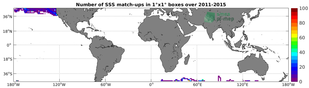
Figure 4: Number of SSS match-ups between Sea mammals SSS and the Aquarius SSS L4 OI v5 - Monthly (IPRC) SSS product for the Mid-Low Latitudes 45N-45S Pi-MEP region over 1°x1° boxes and for the full satellite product period.
