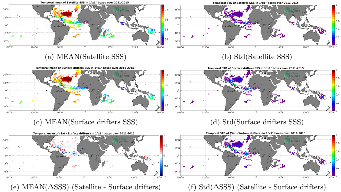
Figure 5: Temporal mean (left) and Std (right) of SSS from Aquarius SSS L4 OI v5 - Monthly (IPRC) (top), Surface drifters in situ dataset (middle), and of \Delta SSS (Satellite - Surface drifters). Only match-up pairs are used to generate these maps.
