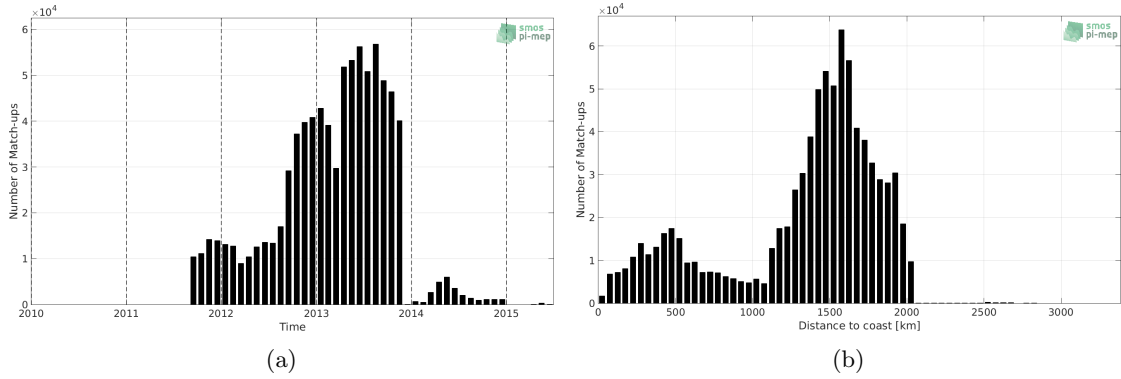
Figure 1: Number of match-ups between Surface drifters and Aquarius-L4-IPRC-V5-MONTHLY SSS as a function of time (a) and as function of the distance to coast (b) over the Mid-Low Latitudes 45N-45S Pi-MEP region and for the full satellite product period.
