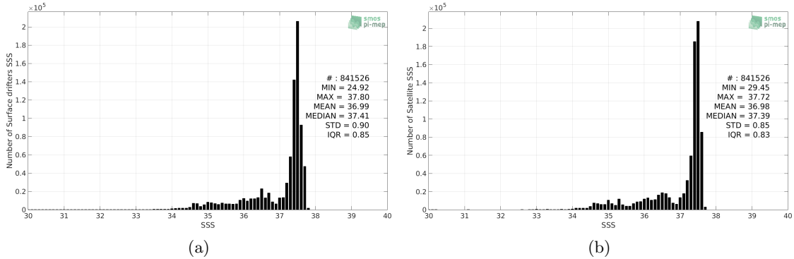
Figure 2: Histograms of SSS from Surface drifters (a) and Aquarius-L4-IPRC-V5-MONTHLY (b) considering all match-up pairs per bins of 0.1 over the Mid-Low Latitudes 45N-45S Pi-MEP region and for the full satellite product period.
