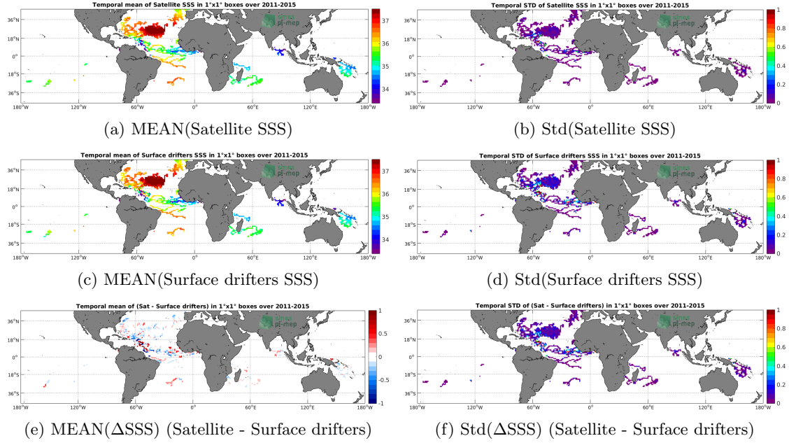
Figure 5: Temporal mean (left) and Std (right) of SSS from Aquarius-L4-IPRC-V5-MONTHLY (top), Surface drifters (middle), and of \Delta SSS (Satellite - Surface drifters). Only match-up pairs are used to generate these maps.
