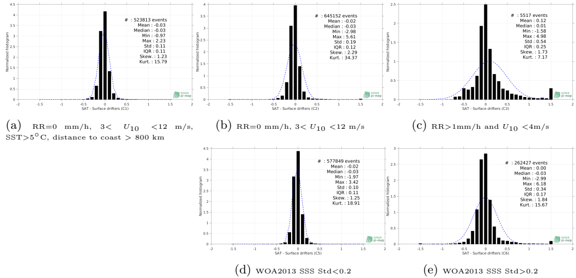
Figure 12: Normalized histogram of \Delta SSS (Aquarius-L4-IPRC-V5-MONTHLY - Surface drifters) for 5 different subdatasets corresponding to: RR=0 mm/h, 3 < U_{10} < 12 m/s, SST > 5^\circ C , distance to coast > 800 km (a), RR=0 mm/h, 3 < U_{10} < 12 m/s (b), RR > 1 mm/h and U_{10} < 4 m/s (c), WOA2013 SSS Std < 0.2 (d), WOA2013 SSS Std > 0.2 (e).
