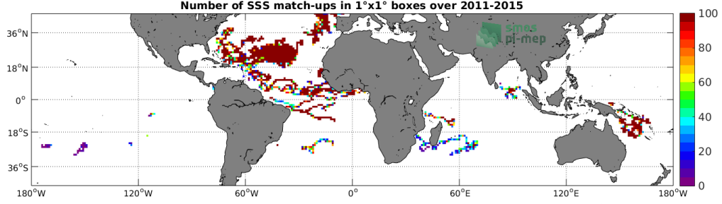
Figure 3: Number of SSS match-ups between Surface drifters SSS and the Aquarius-L4-IPRC-V5-MONTHLY SSS product for the Mid-Low Latitudes 45N-45S Pi-MEP region over 1°x1° boxes and for the full satellite product period.
