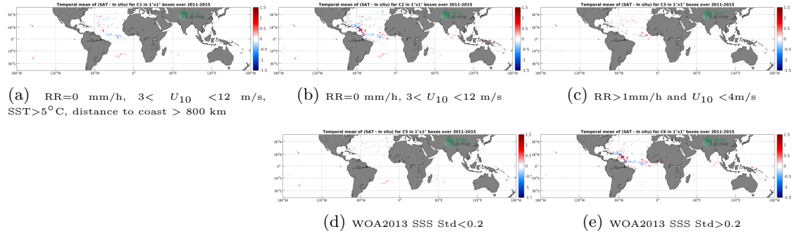
Figure 11: Temporal mean gridded over spatial boxes of size 1^\circ \times 1^\circ of \Delta SSS (Aquarius-L4-IPRC-V5-MONTHLY - Surface drifters) for 5 different subdatasets corresponding to: RR=0 mm/h, 3 < U_{10} < 12 m/s, SST > 5^\circ C , distance to coast > 800 km (a), RR=0 mm/h, 3 < U_{10} < 12 m/s (b), RR > 1 mm/h and U_{10} < 4 m/s (c), WOA2013 SSS Std < 0.2 (d), WOA2013 SSS Std > 0.2 (e).
