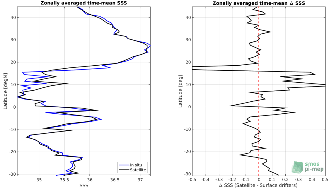
Figure 7: Left panel: Zonal mean SSS from Aquarius-L4-IPRC-V5-MONTHLY satellite product (black) and from Surface drifters (blue). Right panel: Zonal mean of \Delta SSS (Satellite - Surface drifters) for all the collected Pi-MEP match-up pairs estimated over the full satellite product period.
