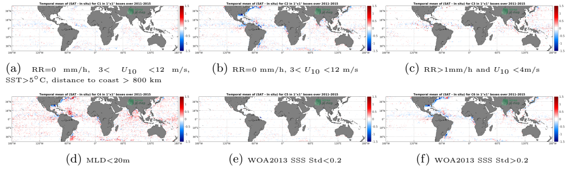
Figure 12: Temporal mean gridded over spatial boxes of size 1^\circ \times 1^\circ of \Delta SSS (Aquarius SSS L4 OI v5 - Monthly (IPRC) - Argo) for 6 different subdatasets corresponding to: RR=0 mm/h, 3 < U_{10} < 12 m/s, SST > 5^\circ C , distance to coast > 800 km (a), RR=0 mm/h, 3 < U_{10} < 12 m/s (b), RR > 1 mm/h and U_{10} < 4 m/s (c), MLD < 20 m (d), WOA2013 SSS Std < 0.2 (e), WOA2013 SSS Std > 0.2 (f).
