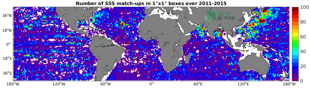
Figure 4: Number of SSS match-ups between Argo SSS and the Aquarius SSS L4 OI v5 - Monthly (IPRC) SSS product for the Mid-Low Latitudes 45N-45S Pi-MEP region over 1^\circ \times 1^\circ boxes and for the full satellite product period.
