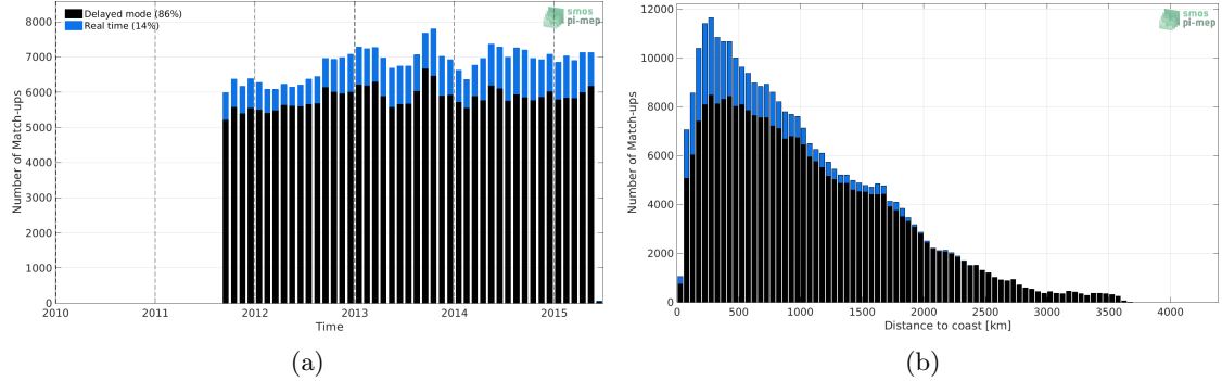
Figure 1: Number of match-ups between Argo and Aquarius SSS L4 OI v5 - Monthly (IPRC) SSS as a function of time (a) and as function of the distance to coast (b) over the Mid-Low Latitudes 45N-45S Pi-MEP region and for the full satellite product period.
