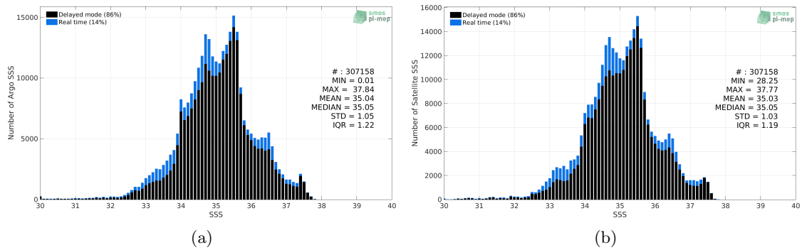
Figure 2: Histograms of SSS from Argo (a) and Aquarius SSS L4 OI v5 - Monthly (IPRC) (b) considering all match-up pairs per bins of 0.1 over the Mid-Low Latitudes 45N-45S Pi-MEP region and for the full satellite product period.
