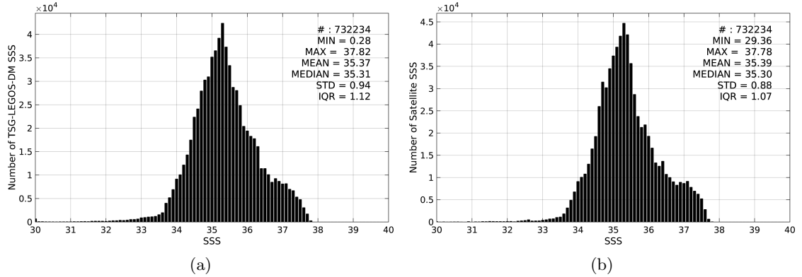
Figure 2: Histograms of SSS from TSG-LEGOS-DM (a) and Aquarius-L4-IPRC-V4-WEEKLY (b) considering all match-up pairs per bins of 0.1 over the Mid-Low Latitudes 45N-45S Pi-MEP region and for the full satellite product period.
