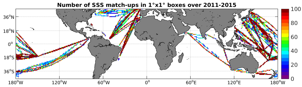
Figure 4: Number of SSS match-ups between TSG-LEGOS-DM SSS and the Aquarius-L4-IPRC-V4-WEEKLY SSS product for the Mid-Low Latitudes 45N-45S Pi-MEP region over 1^\circ \times 1^\circ boxes and for the full satellite product period.
