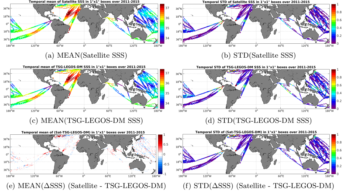
Figure 6: Temporal mean (left) and STD (right) of SSS from Aquarius-L4-IPRC-V4-WEEKLY (top), TSG-LEGOS-DM (middle), and of \Delta SSS (Satellite - TSG-LEGOS-DM). Only match-up pairs are used to generate these maps.
