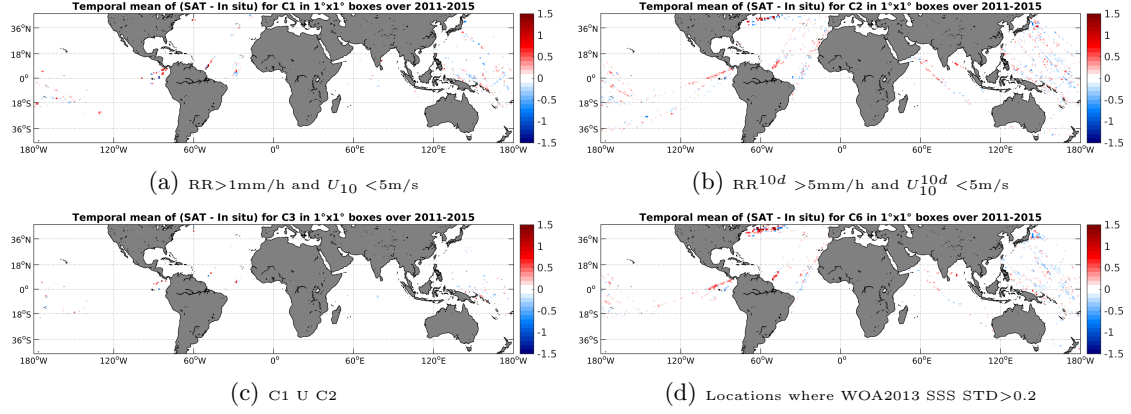
Figure 12: Temporal mean gridded over spatial boxes of size 1^\circ \times 1^\circ of \Delta SSS (Aquarius-L4-IPRC-V4-WEEKLY - TSG-LEGOS-DM) for 4 different subdatasets corresponding to: RR > 1\text{mm/h} and U_{10} < 5\text{m/s} (a), RR^{10d} > 5\text{mm/h} and U_{10}^{10d} < 5\text{m/s} (b), C1 U C2 (c), Locations where WOA2013 SSS STD > 0.2 (d).
