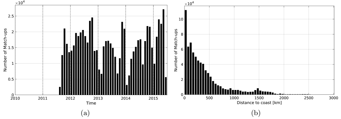
Figure 1: Number of match-ups between TSG-LEGOS-DM and Aquarius-L4-IPRC-V4-WEEKLY SSS as a function of time (a) and as function of the distance to coast (b) over the Mid-Low Latitudes 45N-45S Pi-MEP region and for the full satellite product period.
