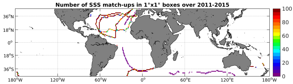
Figure 4: Number of SSS match-ups between TSG-GOSUD-Sailing-ship SSS and the Aquarius-L4-IPRC-V4-WEEKLY SSS product for the Mid-Low Latitudes 45N-45S Pi-MEP region over 1°x1° boxes and for the full satellite product period.
