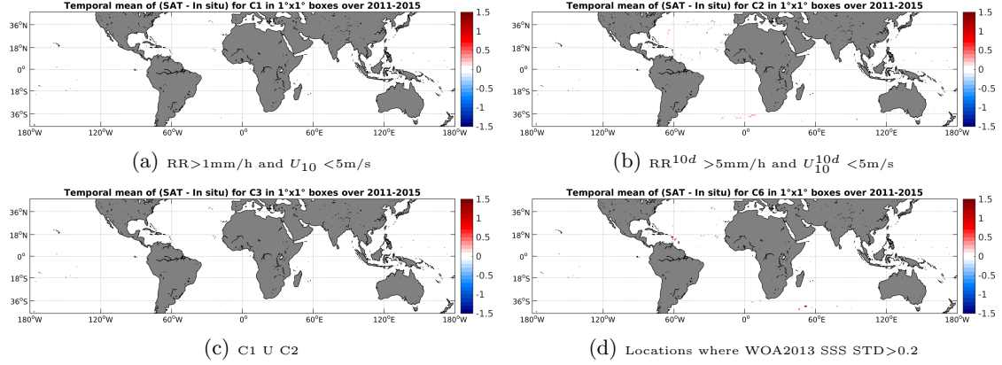
Figure 12: Temporal mean gridded over spatial boxes of size 1^\circ \times 1^\circ of \Delta SSS (Aquarius-L4-IPRC-V4-WEEKLY - TSG-GOSUD-Sailing-ship) for 4 different subdatasets corresponding to: RR > 1 mm/h and U_{10} < 5 m/s (a), RR ^{10d} > 5 mm/h and U_{10}^{10d} < 5 m/s (b), C1 U C2 (c), Locations where WOA2013 SSS STD > 0.2 (d).
