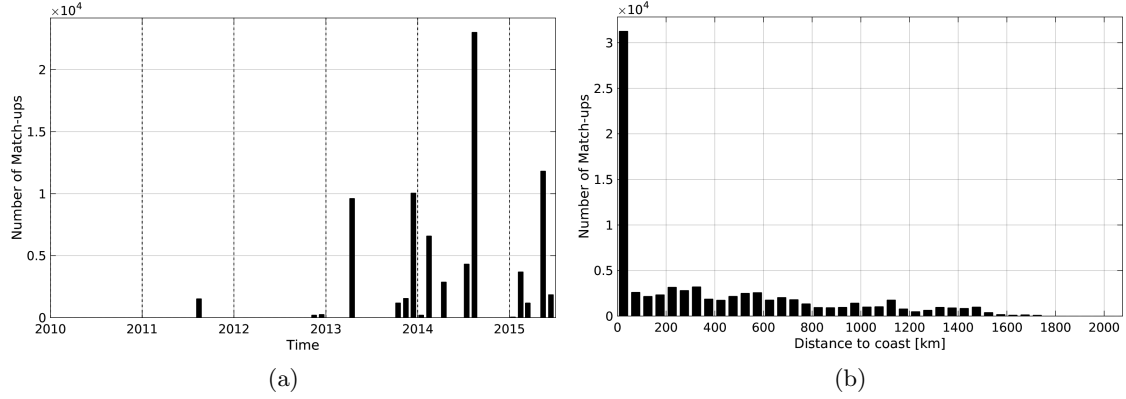
Figure 1: Number of match-ups between TSG-GOSUD-Sailing-ship and Aquarius-L4-IPRC-V4-WEEKLY SSS as a function of time (a) and as function of the distance to coast (b) over the Mid-Low Latitudes 45N-45S Pi-MEP region and for the full satellite product period.
