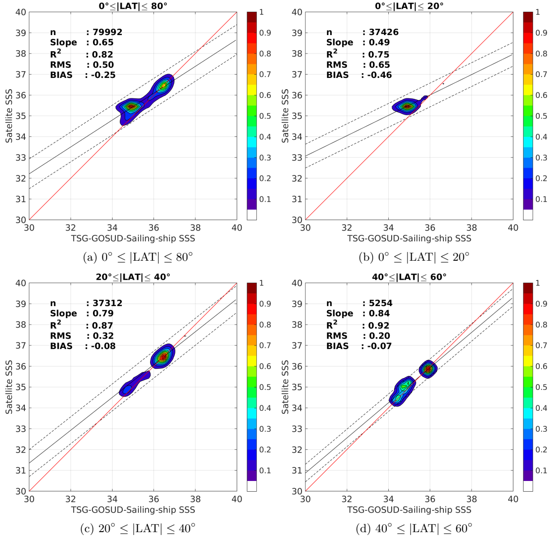
Figure 9: Contour maps of the concentration of Aquarius-L4-IPRC-V4-WEEKLY SSS (y-axis) versus TSG-GOSUD-Sailing-ship SSS (x-axis) at match-up pairs for different latitude bands. For each plot, the red line shows x=y . The black thin and dashed lines indicate a linear fit through the data cloud and the \pm 95\% confidence levels, respectively. The number match-up pairs n , the slope and R^2 coefficient of the linear fit, the root mean square (RMS) and the mean bias between satellite and in situ data are indicated for each latitude band in each plots.
