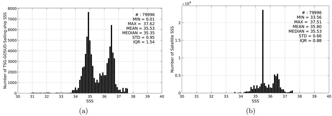
Figure 2: Histograms of SSS from TSG-GOSUD-Sailing-ship (a) and Aquarius-L4-IPRC-V4-WEEKLY (b) considering all match-up pairs per bins of 0.1 over the Mid-Low Latitudes 45N-45S Pi-MEP region and for the full satellite product period.
