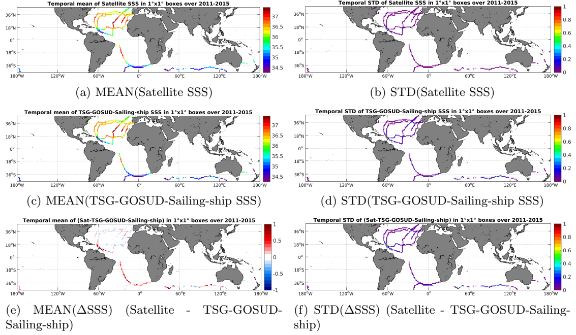
Figure 6: Temporal mean (left) and STD (right) of SSS from Aquarius-L4-IPRC-V4-WEEKLY (top), TSG-GOSUD-Sailing-ship (middle), and of \Delta SSS (Satellite - TSG-GOSUD-Sailing-ship). Only match-up pairs are used to generate these maps.
