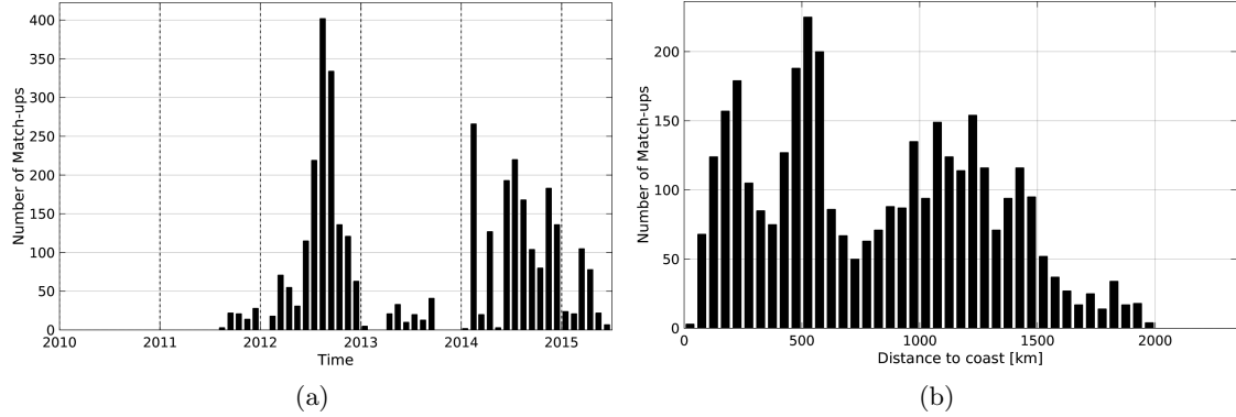
Figure 1: Number of match-ups between Sea mammals and Aquarius-L4-IPRC-V4-WEEKLY SSS as a function of time (a) and as function of the distance to coast (b) over the Mid-Low Latitudes 45N-45S Pi-MEP region and for the full satellite product period.
