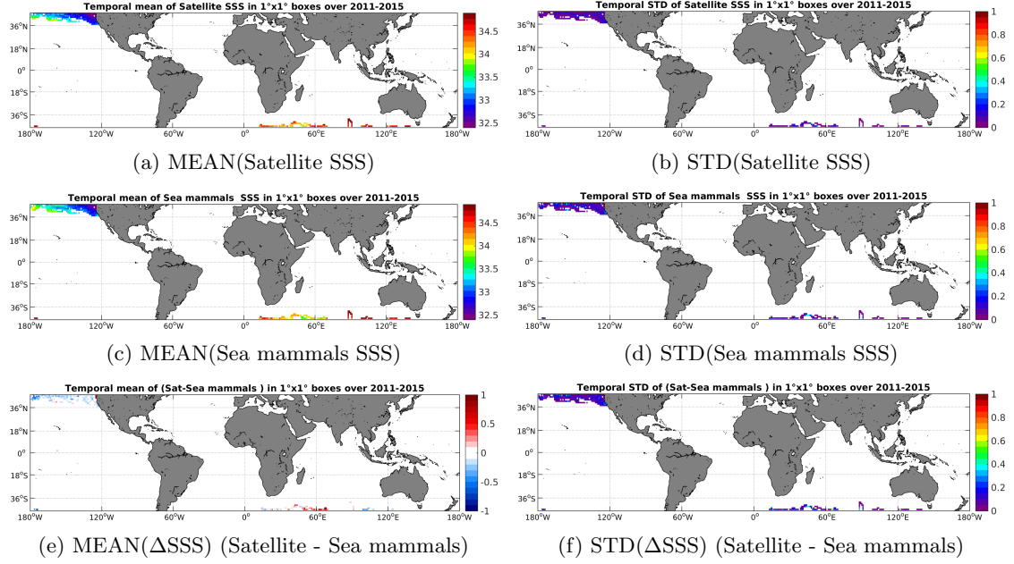
Figure 6: Temporal mean (left) and STD (right) of SSS from Aquarius-L4-IPRC-V4-WEEKLY (top), Sea mammals (middle), and of \Delta SSS (Satellite - Sea mammals). Only match-up pairs are used to generate these maps.
