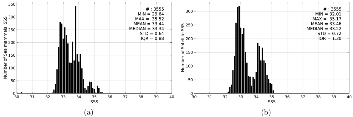
Figure 2: Histograms of SSS from Sea mammals (a) and Aquarius-L4-IPRC-V4-WEEKLY (b) considering all match-up pairs per bins of 0.1 over the Mid-Low Latitudes 45N-45S Pi-MEP region and for the full satellite product period.
