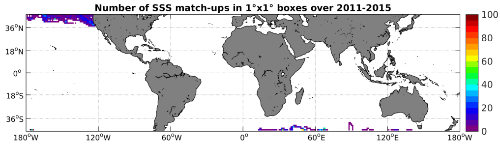
Figure 4: Number of SSS match-ups between Sea mammals SSS and the Aquarius-L4-IPRC-V4-WEEKLY SSS product for the Mid-Low Latitudes 45N-45S Pi-MEP region over 1^\circ \times 1^\circ boxes and for the full satellite product period.
