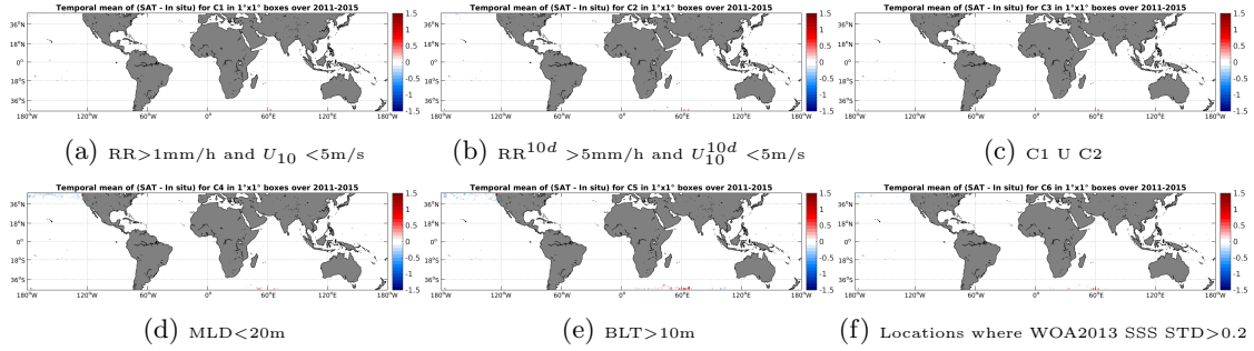
Figure 12: Temporal mean gridded over spatial boxes of size 1^\circ \times 1^\circ of \Delta SSS (Aquarius-L4-IPRC-V4-WEEKLY - Sea mammals) for 6 different subdatasets corresponding to: RR > 1\text{mm/h} and U_{10} < 5\text{m/s} (a), RR^{10d} > 5\text{mm/h} and U_{10}^{10d} < 5\text{m/s} (b), C1 U C2 (c), MLD < 20\text{m} (d), BLT > 10\text{m} (e), Locations where WOA2013 SSS STD > 0.2 (f).
