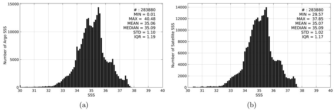
Figure 2: Histograms of SSS from Argo (a) and Aquarius-L4-IPRC-V4-WEEKLY (b) considering all match-up pairs per bins of 0.1 over the Mid-Low Latitudes 45N-45S Pi-MEP region and for the full satellite product period.
