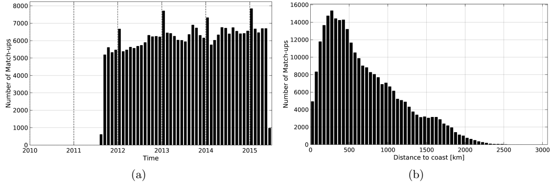
Figure 1: Number of match-ups between Argo and Aquarius-L4-IPRC-V4-WEEKLY SSS as a function of time (a) and as function of the distance to coast (b) over the Mid-Low Latitudes 45N-45S Pi-MEP region and for the full satellite product period.
