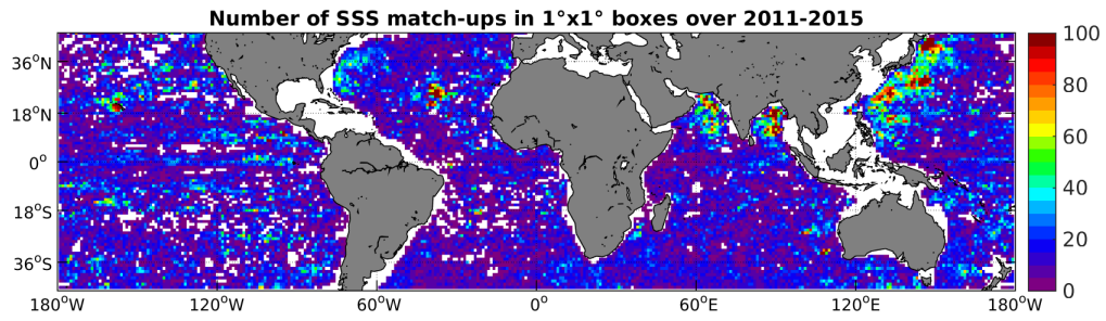
Figure 4: Number of SSS match-ups between Argo SSS and the Aquarius-L4-IPRC-V4-WEEKLY SSS product for the Mid-Low Latitudes 45N-45S Pi-MEP region over 1^\circ \times 1^\circ boxes and for the full satellite product period.
