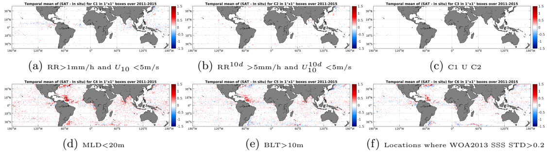
Figure 12: Temporal mean gridded over spatial boxes of size 1^\circ \times 1^\circ of \Delta SSS (Aquarius-L4-IPRC-V4-WEEKLY - Argo) for 6 different subdatasets corresponding to: RR > 1\text{mm/h} and U_{10} < 5\text{m/s} (a), RR^{10d} > 5\text{mm/h} and U_{10}^{10d} < 5\text{m/s} (b), C1 U C2 (c), MLD < 20\text{m} (d), BLT > 10\text{m} (e), Locations where WOA2013 SSS STD > 0.2 (f).
