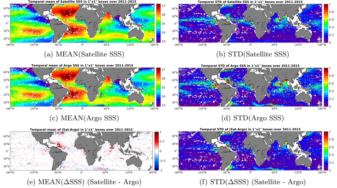
Figure 6: Temporal mean (left) and STD (right) of SSS from Aquarius-L4-IPRC-V4-WEEKLY (top), Argo (middle), and of \Delta SSS (Satellite - Argo). Only match-up pairs are used to generate these maps.
