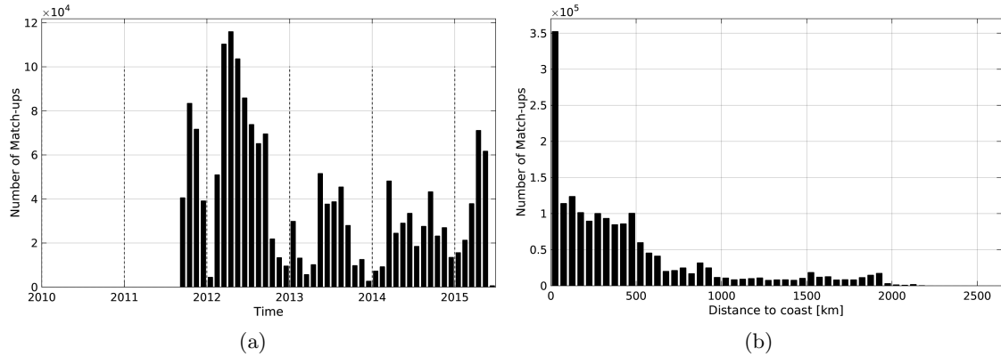
Figure 1: Number of match-ups between TSG-SAMOS and Aquarius-L4-IPRC-V4-MONTHLY SSS as a function of time (a) and as function of the distance to coast (b) over the Mid-Low Latitudes 45N-45S Pi-MEP region and for the full satellite product period.
