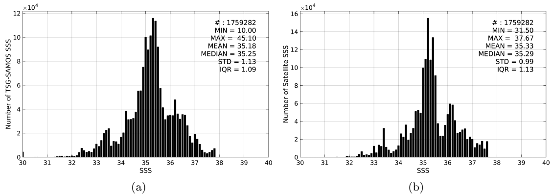
Figure 2: Histograms of SSS from TSG-SAMOS (a) and Aquarius-L4-IPRC-V4-MONTHLY (b) considering all match-up pairs per bins of 0.1 over the Mid-Low Latitudes 45N-45S Pi-MEP region and for the full satellite product period.
