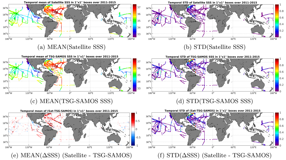
Figure 6: Temporal mean (left) and STD (right) of SSS from Aquarius-L4-IPRC-V4-MONTHLY (top), TSG-SAMOS (middle), and of \Delta SSS (Satellite - TSG-SAMOS). Only match-up pairs are used to generate these maps.
