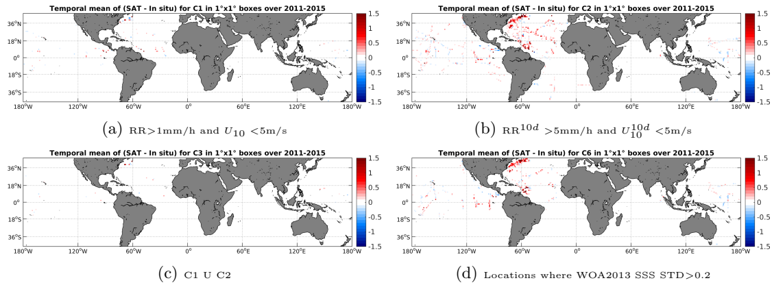
Figure 12: Temporal mean gridded over spatial boxes of size 1^\circ \times 1^\circ of \Delta SSS (Aquarius-L4-IPRC-V4-MONTHLY - TSG-SAMOS) for 4 different subdatasets corresponding to: RR > 1\text{mm/h} and U_{10} < 5\text{m/s} (a), RR^{10d} > 5\text{mm/h} and U_{10}^{10d} < 5\text{m/s} (b), C1 U C2 (c), Locations where WOA2013 SSS STD > 0.2 (d).
