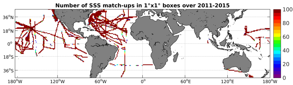
Figure 4: Number of SSS match-ups between TSG-SAMOS SSS and the Aquarius-L4-IPRC-V4-MONTHLY SSS product for the Mid-Low Latitudes 45N-45S Pi-MEP region over 1°x1° boxes and for the full satellite product period.
