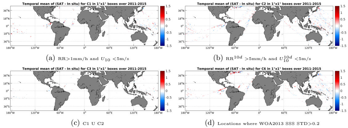
Figure 12: Temporal mean gridded over spatial boxes of size 1^\circ \times 1^\circ of \Delta SSS (Aquarius-L4-IPRC-V4-MONTHLY - TSG-LEGOS-DM) for 4 different subdatasets corresponding to: RR > 1\text{mm/h} and U_{10} < 5\text{m/s} (a), RR^{10d} > 5\text{mm/h} and U_{10}^{10d} < 5\text{m/s} (b), C1 U C2 (c), Locations where WOA2013 SSS STD > 0.2 (d).
