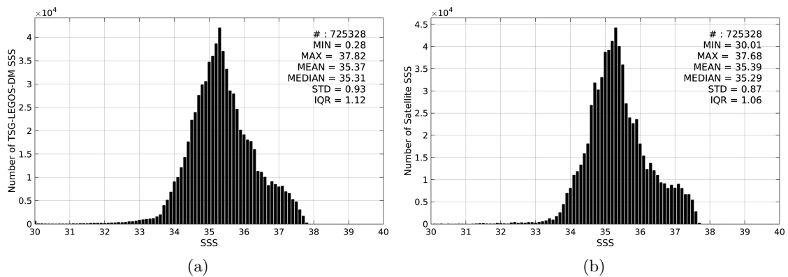
Figure 2: Histograms of SSS from TSG-LEGOS-DM (a) and Aquarius-L4-IPRC-V4-MONTHLY (b) considering all match-up pairs per bins of 0.1 over the Mid-Low Latitudes 45N-45S Pi-MEP region and for the full satellite product period.
