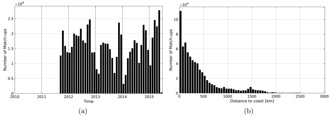
Figure 1: Number of match-ups between TSG-LEGOS-DM and Aquarius-L4-IPRC-V4-MONTHLY SSS as a function of time (a) and as function of the distance to coast (b) over the Mid-Low Latitudes 45N-45S Pi-MEP region and for the full satellite product period.
