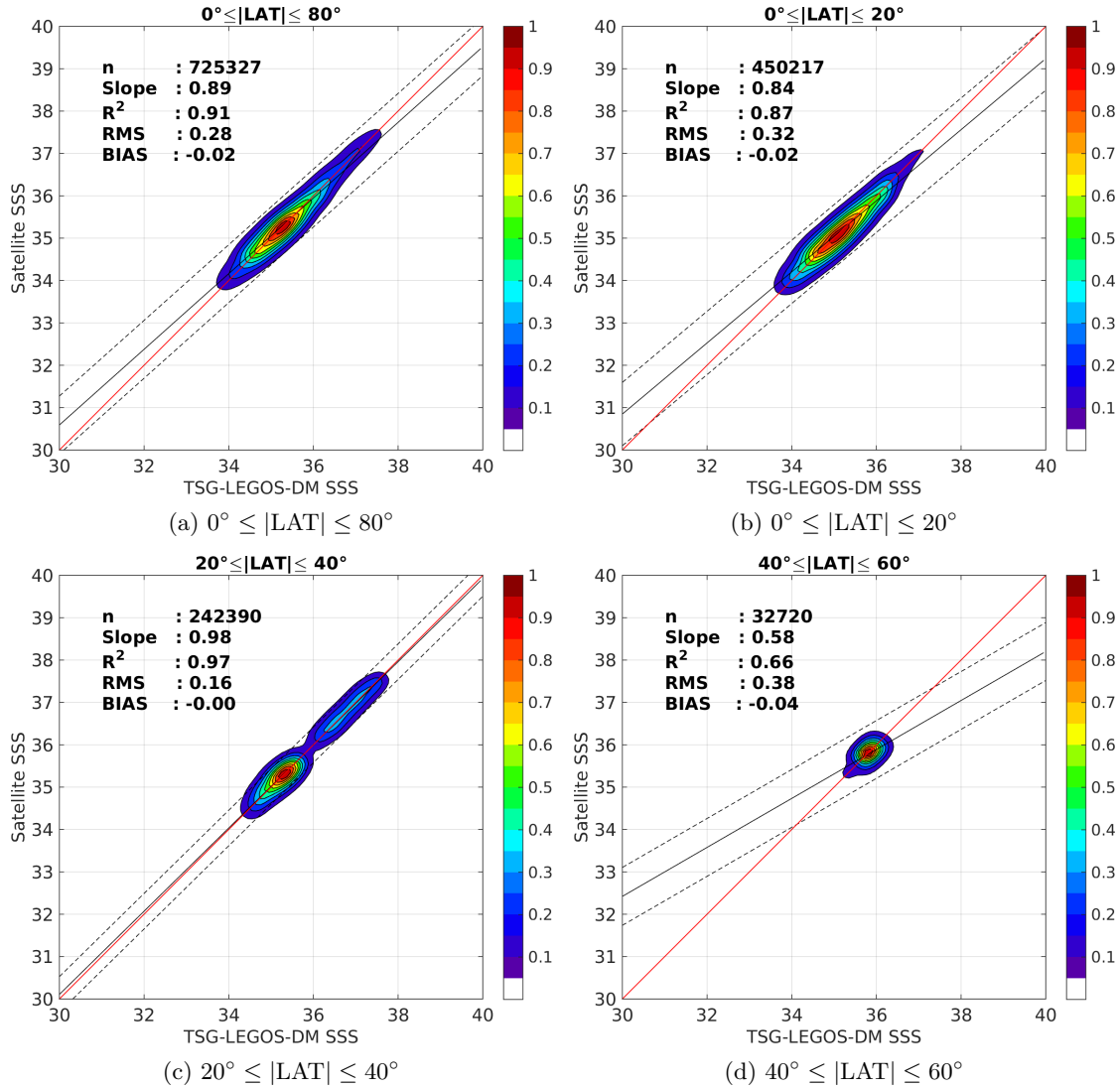
Figure 9: Contour maps of the concentration of Aquarius-L4-IPRC-V4-MONTHLY SSS (y-axis) versus TSG-LEGOS-DM SSS (x-axis) at match-up pairs for different latitude bands. For each plot, the red line shows x=y . The black thin and dashed lines indicate a linear fit through the data cloud and the \pm 95\% confidence levels, respectively. The number match-up pairs n , the slope and R^2 coefficient of the linear fit, the root mean square (RMS) and the mean bias between satellite and in situ data are indicated for each latitude band in each plots.
