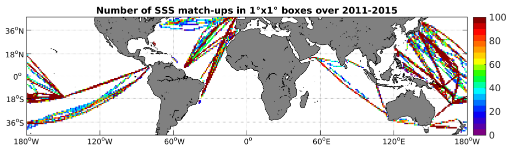
Figure 4: Number of SSS match-ups between TSG-LEGOS-DM SSS and the Aquarius-L4-IPRC-V4-MONTHLY SSS product for the Mid-Low Latitudes 45N-45S Pi-MEP region over 1^\circ \times 1^\circ boxes and for the full satellite product period.
