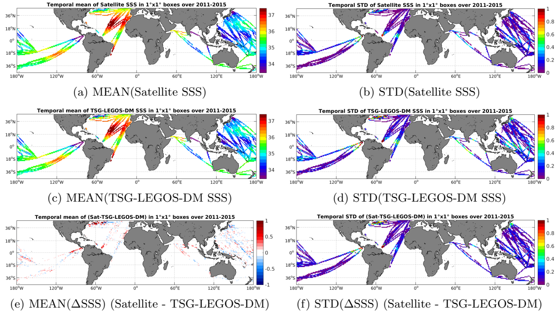
Figure 6: Temporal mean (left) and STD (right) of SSS from Aquarius-L4-IPRC-V4-MONTHLY (top), TSG-LEGOS-DM (middle), and of \Delta SSS (Satellite - TSG-LEGOS-DM). Only match-up pairs are used to generate these maps.
