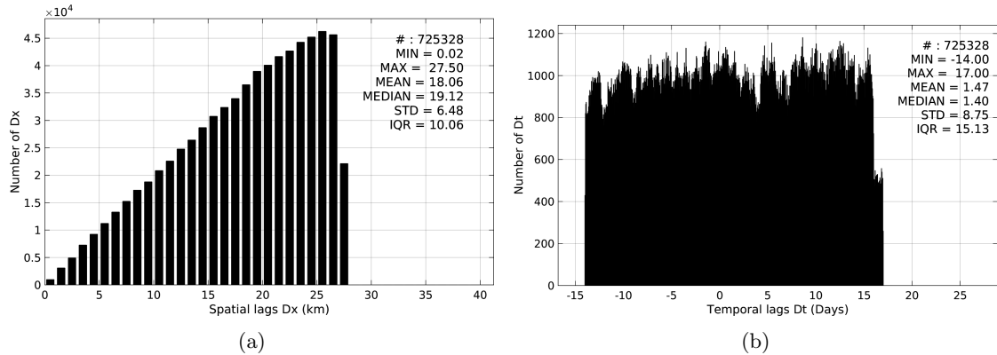
Figure 5: Histograms of the spatial (a) and temporal (b) lags between the time of the TSG-LEGOS-DM measurements and the date of the corresponding Aquarius-L4-IPRC-V4-MONTHLY SSS product.
