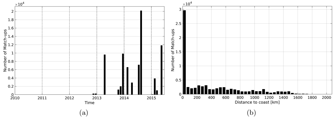
Figure 1: Number of match-ups between TSG-GOSUD-Sailing-ship and Aquarius-L4-IPRC-V4-MONTHLY SSS as a function of time (a) and as function of the distance to coast (b) over the Mid-Low Latitudes 45N-45S Pi-MEP region and for the full satellite product period.
