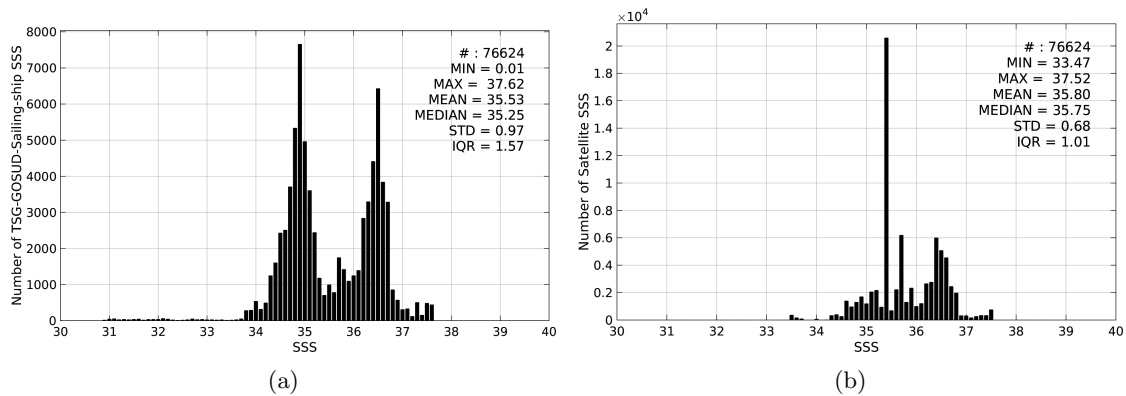
Figure 2: Histograms of SSS from TSG-GOSUD-Sailing-ship (a) and Aquarius-L4-IPRC-V4-MONTHLY (b) considering all match-up pairs per bins of 0.1 over the Mid-Low Latitudes 45N-45S Pi-MEP region and for the full satellite product period.
