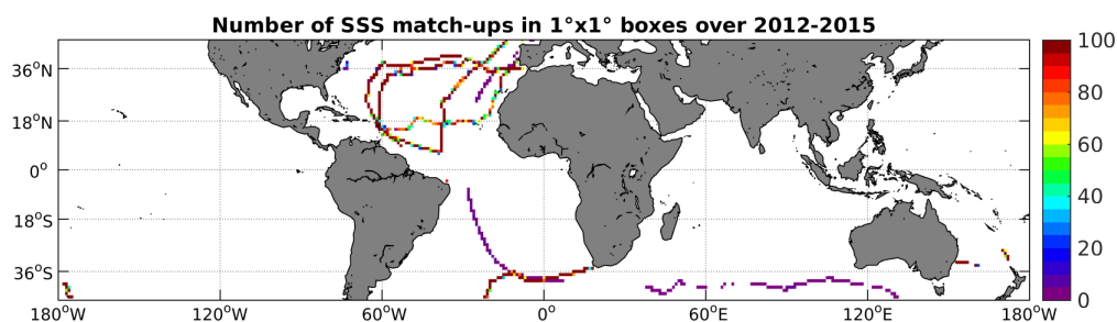
Figure 4: Number of SSS match-ups between TSG-GOSUD-Sailing-ship SSS and the Aquarius-L4-IPRC-V4-MONTHLY SSS product for the Mid-Low Latitudes 45N-45S Pi-MEP region over 1^\circ \times 1^\circ boxes and for the full satellite product period.
