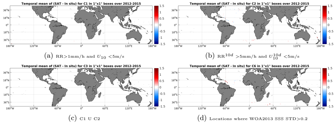
Figure 12: Temporal mean gridded over spatial boxes of size 1^\circ \times 1^\circ of \Delta SSS (Aquarius-L4-IPRC-V4-MONTHLY - TSG-GOSUD-Sailing-ship) for 4 different subdatasets corresponding to: RR > 1 mm/h and U_{10} < 5 m/s (a), RR ^{10d} > 5 mm/h and U_{10}^{10d} < 5 m/s (b), C1 U C2 (c), Locations where WOA2013 SSS STD > 0.2 (d).
