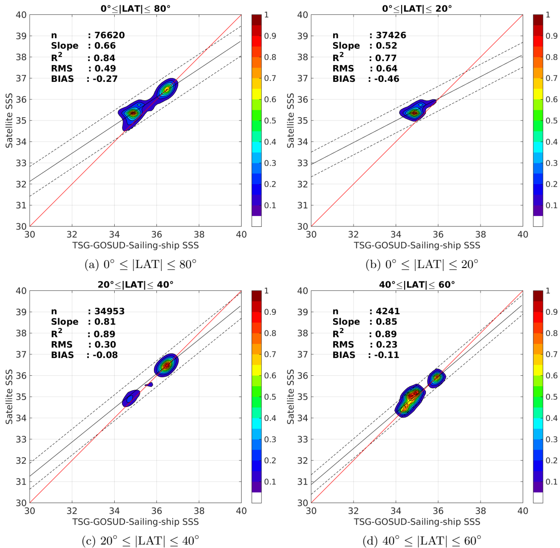
Figure 9: Contour maps of the concentration of Aquarius-L4-IPRC-V4-MONTHLY SSS (y-axis) versus TSG-GOSUD-Sailing-ship SSS (x-axis) at match-up pairs for different latitude bands. For each plot, the red line shows x=y . The black thin and dashed lines indicate a linear fit through the data cloud and the \pm 95\% confidence levels, respectively. The number match-up pairs n , the slope and R^2 coefficient of the linear fit, the root mean square (RMS) and the mean bias between satellite and in situ data are indicated for each latitude band in each plots.
