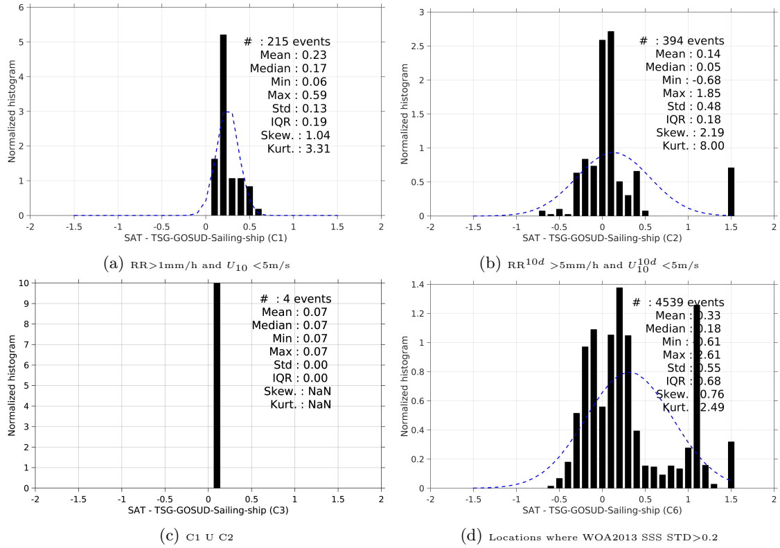
Figure 13: Normalized histogram of \Delta\text{SSS} (Aquarius-L4-IPRC-V4-MONTHLY - TSG-GOSUD-Sailing-ship) for 6 different subdatasets corresponding to: RR > 1mm/h and U_{10} < 5\text{m/s} (a), RR^{10d} > 5\text{mm/h} and U_{10}^{10d} < 5\text{m/s} (b), C1 U C2 (c), Locations where WOA2013 SSS STD > 0.2 (d).
