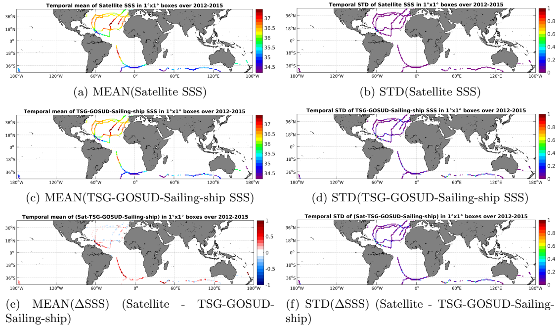
Figure 6: Temporal mean (left) and STD (right) of SSS from Aquarius-L4-IPRC-V4-MONTHLY (top), TSG-GOSUD-Sailing-ship (middle), and of \Delta SSS (Satellite - TSG-GOSUD-Sailing-ship). Only match-up pairs are used to generate these maps.
