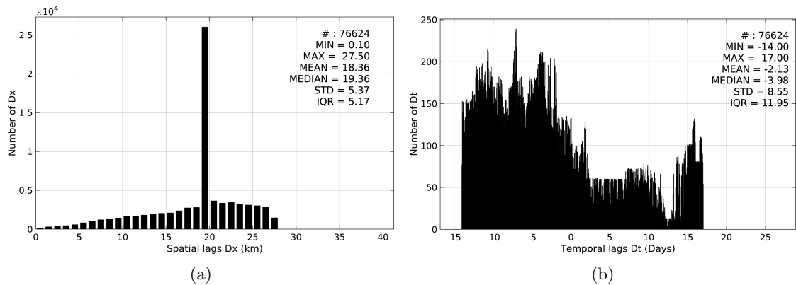
Figure 5: Histograms of the spatial (a) and temporal (b) lags between the time of the TSG-GOSUD-Sailing-ship measurements and the date of the corresponding Aquarius-L4-IPRC-V4-MONTHLY SSS product.
