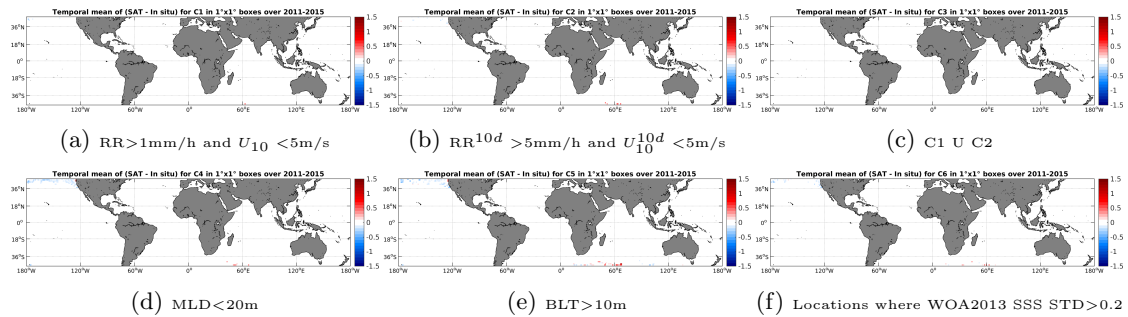
Figure 12: Temporal mean gridded over spatial boxes of size 1^\circ \times 1^\circ of \Delta SSS (Aquarius-L4-IPRC-V4-MONTHLY - Sea mammals) for 6 different subdatasets corresponding to: RR>1mm/h and U_{10} < 5\text{m/s} (a), RR^{10d} > 5\text{mm/h} and U_{10}^{10d} < 5\text{m/s} (b), C1 U C2 (c), MLD<20m (d), BLT>10m (e), Locations where WOA2013 SSS STD>0.2 (f).
