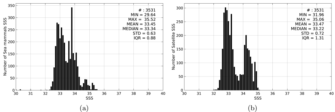
Figure 2: Histograms of SSS from Sea mammals (a) and Aquarius-L4-IPRC-V4-MONTHLY (b) considering all match-up pairs per bins of 0.1 over the Mid-Low Latitudes 45N-45S Pi-MEP region and for the full satellite product period.
