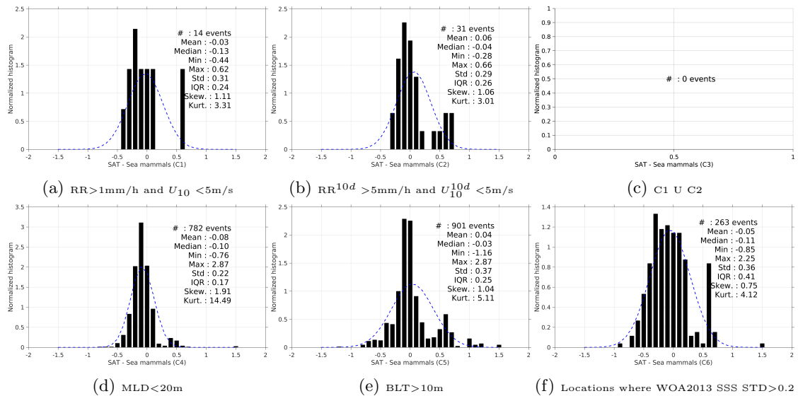
Figure 13: Normalized histogram of \Delta SSS (Aquarius-L4-IPRC-V4-MONTHLY - Sea mammals) for 6 different subdatasets corresponding to: RR>1mm/h and U_{10} < 5\text{m/s} (a), RR^{10d} > 5\text{mm/h} and U_{10}^{10d} < 5\text{m/s} (b), C1 U C2 (c), MLD<20m (d), BLT>10m (e), Locations where WOA2013 SSS STD>0.2 (f).
