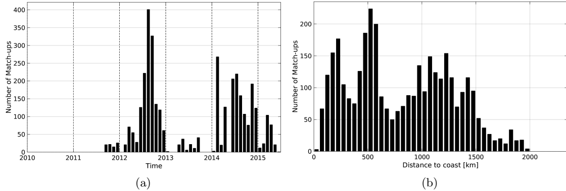
Figure 1: Number of match-ups between Sea mammals and Aquarius-L4-IPRC-V4-MONTHLY SSS as a function of time (a) and as function of the distance to coast (b) over the Mid-Low Latitudes 45N-45S Pi-MEP region and for the full satellite product period.
