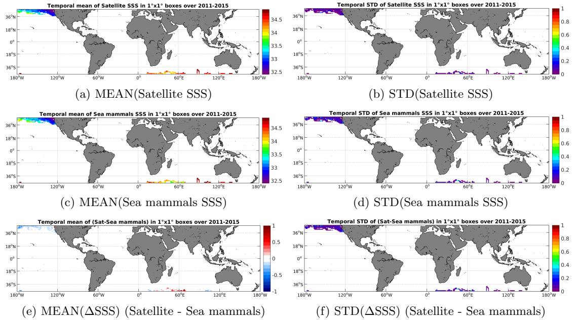
Figure 6: Temporal mean (left) and STD (right) of SSS from Aquarius-L4-IPRC-V4-MONTHLY (top), Sea mammals (middle), and of \Delta SSS (Satellite - Sea mammals). Only match-up pairs are used to generate these maps.
