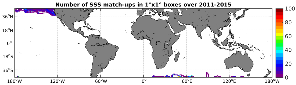
Figure 4: Number of SSS match-ups between Sea mammals SSS and the Aquarius-L4-IPRC-V4-MONTHLY SSS product for the Mid-Low Latitudes 45N-45S Pi-MEP region over 1^\circ \times 1^\circ boxes and for the full satellite product period.
