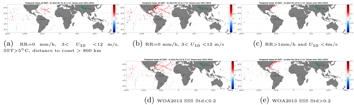
Figure 12: Temporal mean gridded over spatial boxes of size 1^\circ \times 1^\circ of \Delta\text{SSS} (Aquarius SSS L3 OR v5 - 7-Day running (NASA-GSFC) - TSG (SAMOS)) for 5 different subdatasets corresponding to:RR=0 mm/h, 3 < U_{10} < 12 m/s, SST >5^\circ\text{C} , distance to coast > 800 km (a), RR=0 mm/h, 3 < U_{10} < 12 m/s (b), RR >1 mm/h and U_{10} < 4 m/s (c), WOA2013 SSS Std <0.2 (d), WOA2013 SSS Std >0.2 (e).
