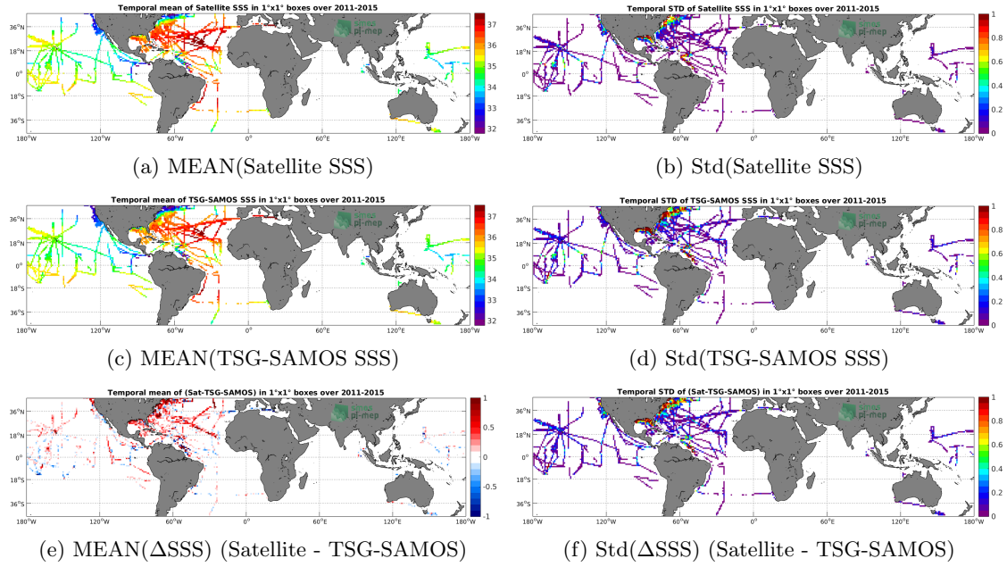
Figure 6: Temporal mean (left) and Std (right) of SSS from Aquarius-L3-OR-V5-7DAY-RUNNING-1DEG (top), TSG-SAMOS (middle), and of \Delta SSS (Satellite - TSG-SAMOS). Only match-up pairs are used to generate these maps.
