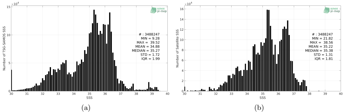
Figure 2: Histograms of SSS from TSG-SAMOS (a) and Aquarius-L3-OR-V5-7DAY-RUNNING-1DEG (b) considering all match-up pairs per bins of 0.1 over the Mid-Low Latitudes 45N-45S Pi-MEP region and for the full satellite product period.
