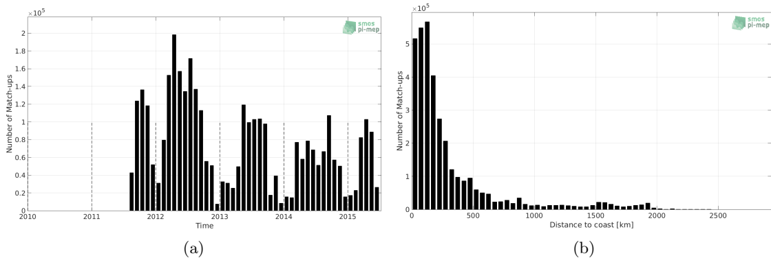
Figure 1: Number of match-ups between TSG-SAMOS and Aquarius-L3-OR-V5-7DAY-RUNNING-1DEG SSS as a function of time (a) and as function of the distance to coast (b) over the Mid-Low Latitudes 45N-45S Pi-MEP region and for the full satellite product period.
