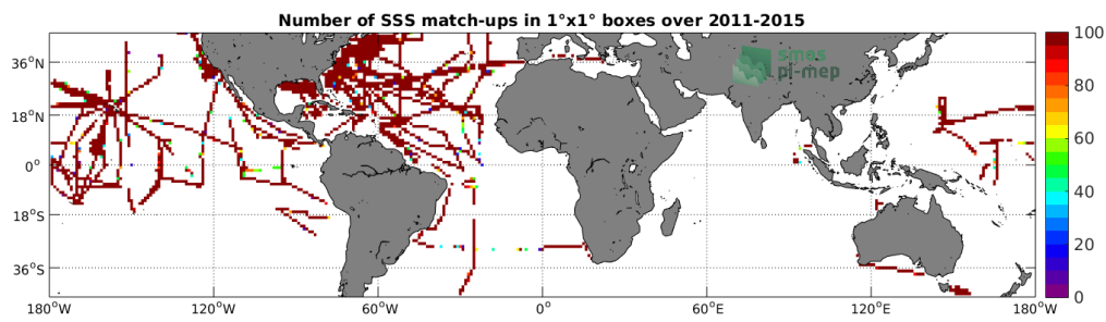
Figure 4: Number of SSS match-ups between TSG-SAMOS SSS and the Aquarius-L3-OR-V5-7DAY-RUNNING-1DEG SSS product for the Mid-Low Latitudes 45N-45S Pi-MEP region over 1^\circ \times 1^\circ boxes and for the full satellite product period.
