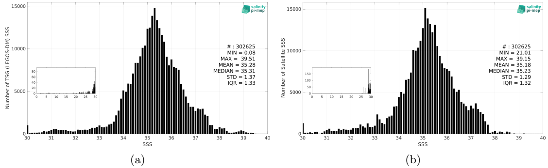
Figure 3: Histograms of SSS from TSG (LEGOS-DM) (a) and Aquarius SSS L3 OR v5 - 7-Day running (NASA-GSFC) (b) considering all match-up pairs per bins of 0.1 over the Mid-Low Latitudes 45N-45S Pi-MEP region and for the full satellite product period.
