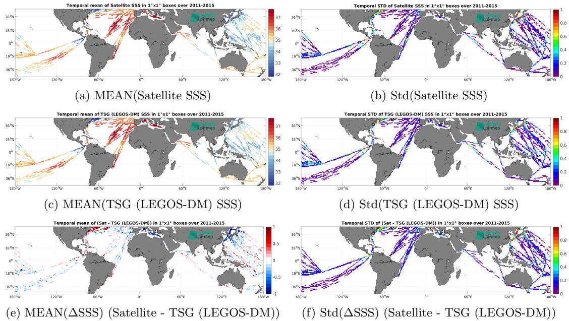
Figure 7: Temporal mean (left) and Std (right) of SSS from Aquarius SSS L3 OR v5 - 7-Day running (NASA-GSFC) (top), TSG (LEGOS-DM) (middle), and of \Delta SSS (Satellite - TSG (LEGOS-DM)). Only match-up pairs are used to generate these maps.
