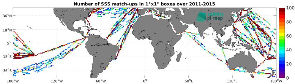
Figure 5: Number of SSS match-ups between TSG (LEGOS-DM) SSS and the Aquarius SSS L3 OR v5 - 7-Day running (NASA-GSFC) SSS product for the Mid-Low Latitudes 45N-45S Pi-MEP region over 1^\circ \times 1^\circ boxes and for the full satellite product period.
