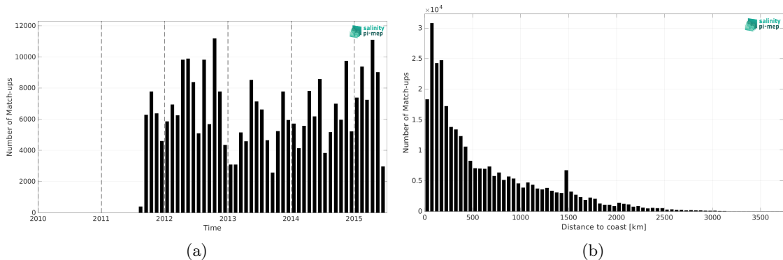
Figure 2: Number of match-ups between TSG (LEGOS-DM) and Aquarius SSS L3 OR v5 - 7-Day running (NASA-GSFC) SSS as a function of time (a) and as function of the distance to coast (b) over the Mid-Low Latitudes 45N-45S Pi-MEP region and for the full satellite product period.
