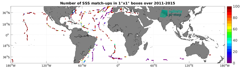
Figure 5: Number of SSS match-ups between TSG (GOSUD-Sailing-ship) SSS and the Aquarius SSS L3 OR v5 - 7-Day running (NASA-GSFC) SSS product for the Mid-Low Latitudes 45N-45S Pi-MEP region over 1^\circ \times 1^\circ boxes and for the full satellite product period.
