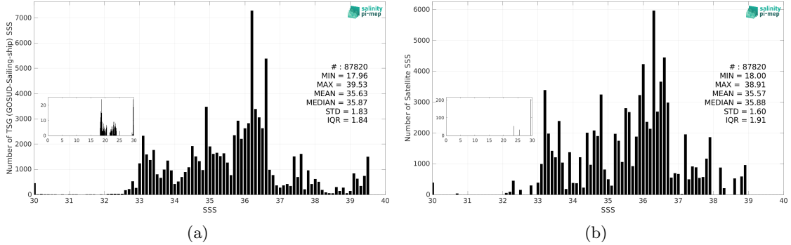
Figure 3: Histograms of SSS from TSG (GOSUD-Sailing-ship) (a) and Aquarius SSS L3 OR v5 - 7-Day running (NASA-GSFC) (b) considering all match-up pairs per bins of 0.1 over the Mid-Low Latitudes 45N-45S Pi-MEP region and for the full satellite product period.
