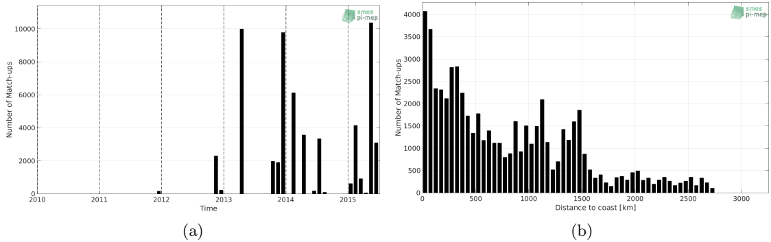
Figure 1: Number of match-ups between TSG-GOSUD-Sailing-ship and Aquarius-L3-OR-V5-7DAY-RUNNING-1DEG SSS as a function of time (a) and as function of the distance to coast (b) over the Mid-Low Latitudes 45N-45S Pi-MEP region and for the full satellite product period.
