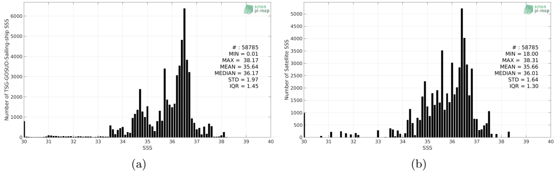
Figure 2: Histograms of SSS from TSG-GOSUD-Sailing-ship (a) and Aquarius-L3-OR-V5-7DAY-RUNNING-1DEG (b) considering all match-up pairs per bins of 0.1 over the Mid-Low Latitudes 45N-45S Pi-MEP region and for the full satellite product period.
