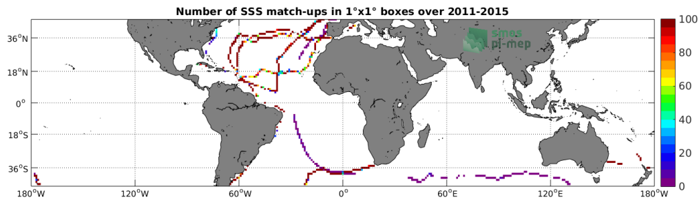
Figure 4: Number of SSS match-ups between TSG-GOSUD-Sailing-ship SSS and the Aquarius-L3-OR-V5-7DAY-RUNNING-1DEG SSS product for the Mid-Low Latitudes 45N-45S Pi-MEP region over 1^\circ \times 1^\circ boxes and for the full satellite product period.
