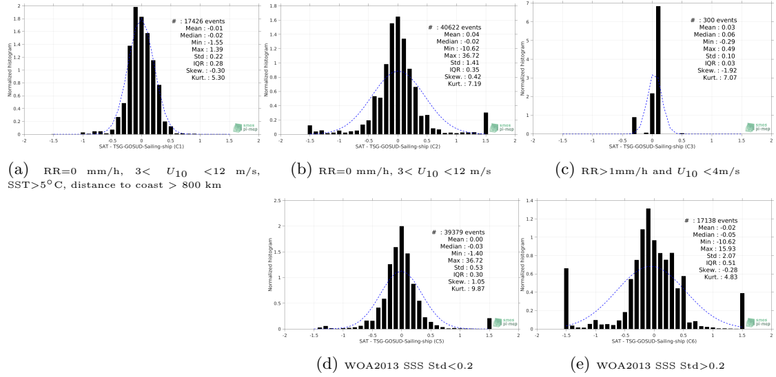
Figure 13: Normalized histogram of \Delta\text{SSS} (Aquarius-L3-OR-V5-7DAY-RUNNING-1DEG - TSG-GOSUD-Sailing-ship) for 5 different subdatasets corresponding to: RR=0 mm/h, 3 < U_{10} < 12 m/s, SST > 5^{\circ}\text{C} , distance to coast > 800 km (a), RR=0 mm/h, 3 < U_{10} < 12 m/s (b), RR > 1\text{mm/h} and U_{10} < 4\text{m/s} (c), WOA2013 SSS Std < 0.2 (d), WOA2013 SSS Std > 0.2 (e).
