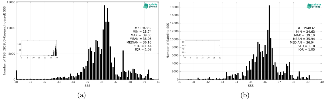
Figure 3: Histograms of SSS from TSG (GOSUD-Research-vessel) (a) and Aquarius SSS L3 OR v5 - 7-Day running (NASA-GSFC) (b) considering all match-up pairs per bins of 0.1 over the Mid-Low Latitudes 45N-45S Pi-MEP region and for the full satellite product period.
