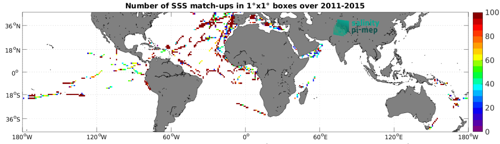
Figure 5: Number of SSS match-ups between TSG (GOSUD-Research-vessel) SSS and the Aquarius SSS L3 OR v5 - 7-Day running (NASA-GSFC) SSS product for the Mid-Low Latitudes 45N-45S Pi-MEP region over 1^\circ \times 1^\circ boxes and for the full satellite product period.
