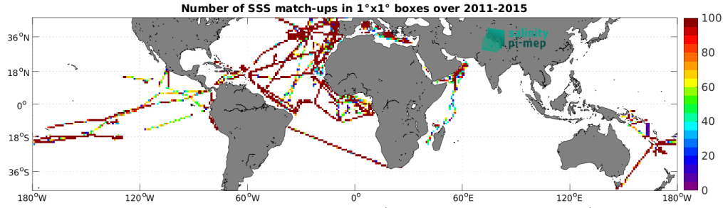
Figure 4: Number of SSS match-ups between TSG (GOSUD-Research-vessel) SSS and the Aquarius SSS L3 OR v5 - 7-Day running (NASA-GSFC) SSS product for the Mid-Low Latitudes 45N-45S Pi-MEP region over 1^\circ \times 1^\circ boxes and for the full satellite product period.
