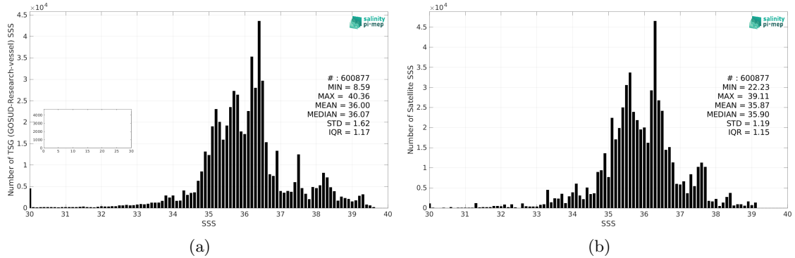
Figure 2: Histograms of SSS from TSG (GOSUD-Research-vessel) (a) and Aquarius SSS L3 OR v5 - 7-Day running (NASA-GSFC) (b) considering all match-up pairs per bins of 0.1 over the Mid-Low Latitudes 45N-45S Pi-MEP region and for the full satellite product period.
