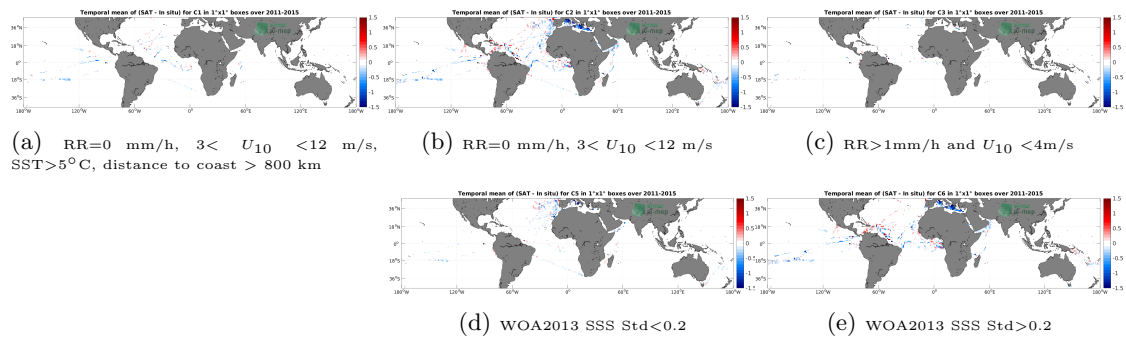
Figure 12: Temporal mean gridded over spatial boxes of size 1^\circ \times 1^\circ of \Delta\text{SSS} (Aquarius SSS L3 OR v5 - 7-Day running (NASA-GSFC) - TSG (GOSUD-Research-vessel)) for 5 different subdatasets corresponding to:RR=0 mm/h, 3 < U_{10} < 12 m/s, SST >5^\circ\text{C} , distance to coast > 800 km (a), RR=0 mm/h, 3 < U_{10} < 12 m/s (b), RR >1 mm/h and U_{10} < 4 m/s (c), WOA2013 SSS Std <0.2 (d), WOA2013 SSS Std >0.2 (e).
