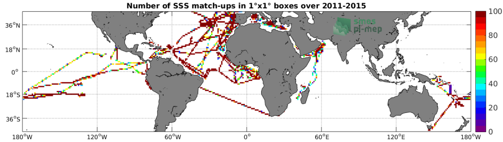
Figure 4: Number of SSS match-ups between TSG-GOSUD-Research-vessel SSS and the Aquarius-L3-OR-V5-7DAY-RUNNING-1DEG SSS product for the Mid-Low Latitudes 45N-45S Pi-MEP region over 1^{\circ} \times 1^{\circ} boxes and for the full satellite product period.
