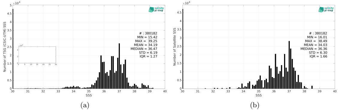
Figure 2: Histograms of SSS from TSG (CSIC-UTM) (a) and Aquarius SSS L3 OR v5 - 7-Day running (NASA-GSFC) (b) considering all match-up pairs per bins of 0.1 over the Mid-Low Latitudes 45N-45S Pi-MEP region and for the full satellite product period.
