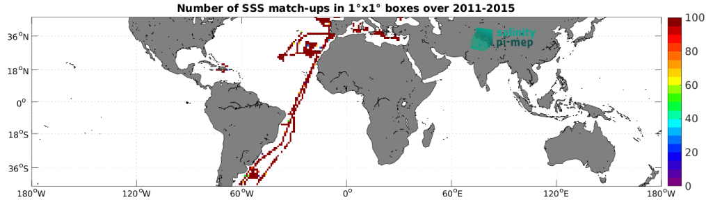
Figure 4: Number of SSS match-ups between TSG (CSIC-UTM) SSS and the Aquarius SSS L3 OR v5 - 7-Day running (NASA-GSFC) SSS product for the Mid-Low Latitudes 45N-45S Pi-MEP region over 1^\circ \times 1^\circ boxes and for the full satellite product period.
