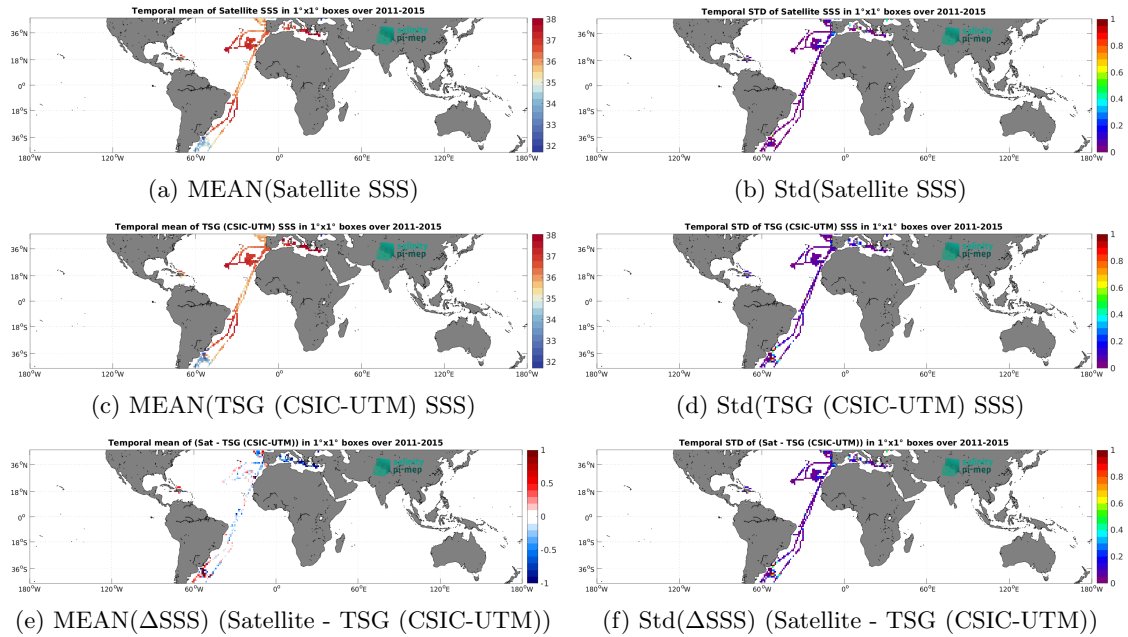
Figure 6: Temporal mean (left) and Std (right) of SSS from Aquarius SSS L3 OR v5 - 7-Day running (NASA-GSFC) (top), TSG (CSIC-UTM) (middle), and of \Delta SSS (Satellite - TSG (CSIC-UTM)). Only match-up pairs are used to generate these maps.
