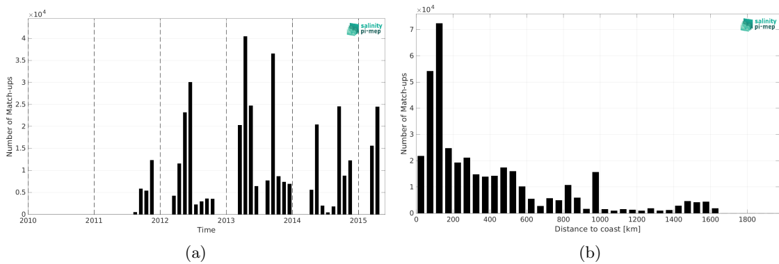
Figure 1: Number of match-ups between TSG (CSIC-UTM) and Aquarius SSS L3 OR v5 - 7-Day running (NASA-GSFC) SSS as a function of time (a) and as function of the distance to coast (b) over the Mid-Low Latitudes 45N-45S Pi-MEP region and for the full satellite product period.
