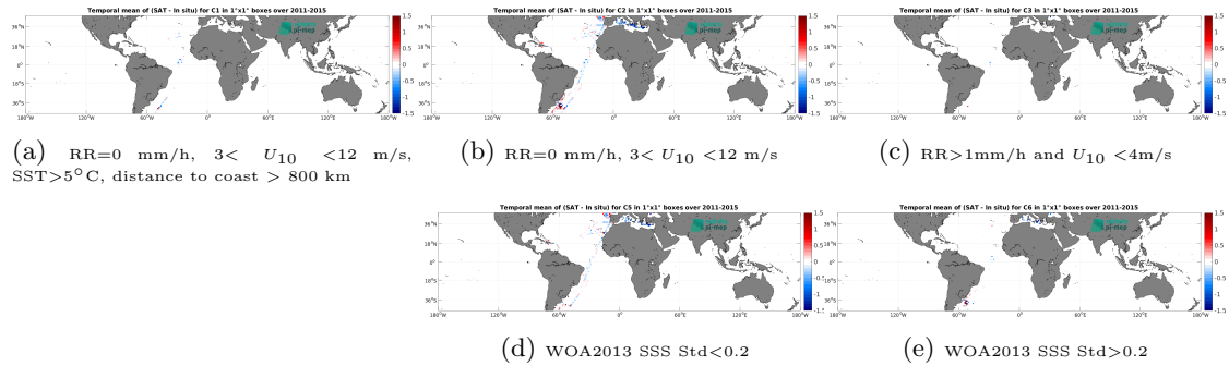
Figure 12: Temporal mean gridded over spatial boxes of size 1^\circ \times 1^\circ of \Delta SSS (Aquarius SSS L3 OR v5 - 7-Day running (NASA-GSFC) - TSG (CSIC-UTM)) for 5 different subdatasets corresponding to:RR=0 mm/h, 3 < U_{10} < 12 m/s, SST >5^\circ C, distance to coast > 800 km (a), RR=0 mm/h, 3 < U_{10} < 12 m/s (b), RR >1 mm/h and U_{10} < 4 m/s (c), WOA2013 SSS Std <0.2 (d), WOA2013 SSS Std >0.2 (e).
