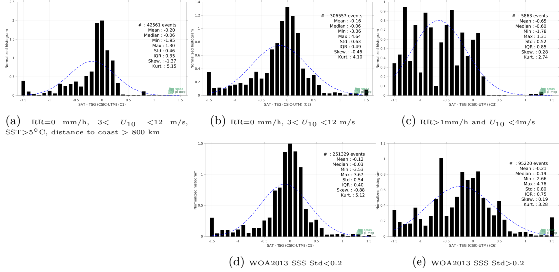
Figure 13: Normalized histogram of \Delta\text{SSS} (Aquarius SSS L3 OR v5 - 7-Day running (NASA-GSFC) - TSG (CSIC-UTM)) for 5 different subdatasets corresponding to: RR=0 mm/h, 3 < U_{10} < 12 m/s, SST > 5^\circ\text{C} , distance to coast > 800 km (a), RR=0 mm/h, 3 < U_{10} < 12 m/s (b), RR > 1 mm/h and U_{10} < 4 m/s (c), WOA2013 SSS Std < 0.2 (d), WOA2013 SSS Std > 0.2 (e).
