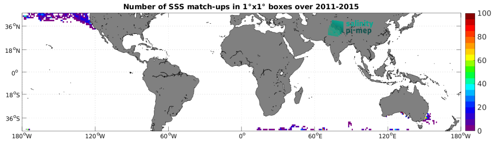
Figure 5: Number of SSS match-ups between Marine mammals SSS and the Aquarius SSS L3 OR v5 - 7-Day running (NASA-GSFC) SSS product for the Mid-Low Latitudes 45N-45S Pi-MEP region over 1^\circ \times 1^\circ boxes and for the full satellite product period.
