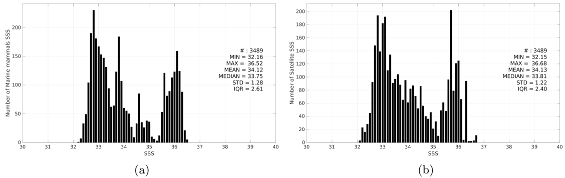
Figure 3: Histograms of SSS from Marine mammals (a) and Aquarius SSS L3 OR v5 - 7-Day running (NASA-GSFC) (b) considering all match-up pairs per bins of 0.1 over the Mid-Low Latitudes 45N-45S Pi-MEP region and for the full satellite product period.
