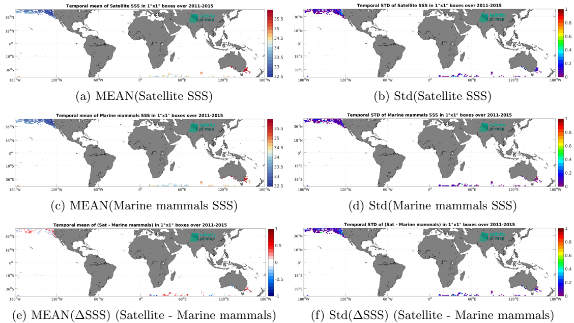
Figure 7: Temporal mean (left) and Std (right) of SSS from Aquarius SSS L3 OR v5 - 7-Day running (NASA-GSFC) (top), Marine mammals (middle), and of \Delta SSS (Satellite - Marine mammals). Only match-up pairs are used to generate these maps.
