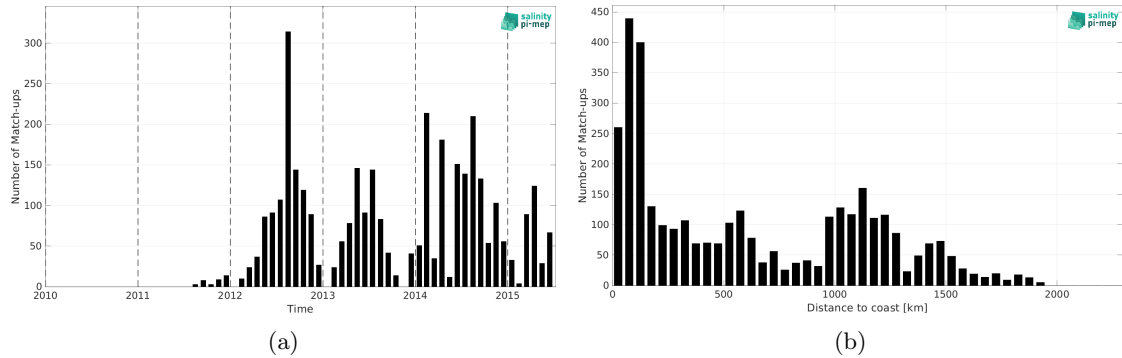
Figure 2: Number of match-ups between Marine mammals and Aquarius SSS L3 OR v5 - 7-Day running (NASA-GSFC) SSS as a function of time (a) and as function of the distance to coast (b) over the Mid-Low Latitudes 45N-45S Pi-MEP region and for the full satellite product period.
