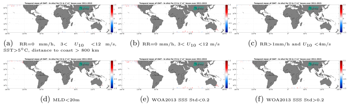
Figure 14: Temporal mean gridded over spatial boxes of size 1^\circ \times 1^\circ of \Delta SSS (Aquarius SSS L3 OR v5 - 7-Day running (NASA-GSFC) - Marine mammals) for 6 different subdatasets corresponding to:RR=0 mm/h, 3 < U_{10} < 12 m/s, SST>5°C, distance to coast > 800 km (a), RR=0 mm/h, 3 < U_{10} < 12 m/s (b), RR>1mm/h and U_{10} < 4 m/s (c),MLD<20m (d),WOA2013 SSS Std<0.2 (e),WOA2013 SSS Std>0.2 (f).
