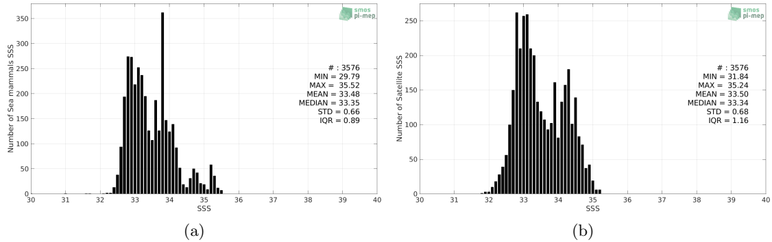
Figure 2: Histograms of SSS from Sea mammals (a) and Aquarius SSS L3 OR v5 - 7-Day running (NASA-GSFC) (b) considering all match-up pairs per bins of 0.1 over the Mid-Low Latitudes 45N-45S Pi-MEP region and for the full satellite product period.
