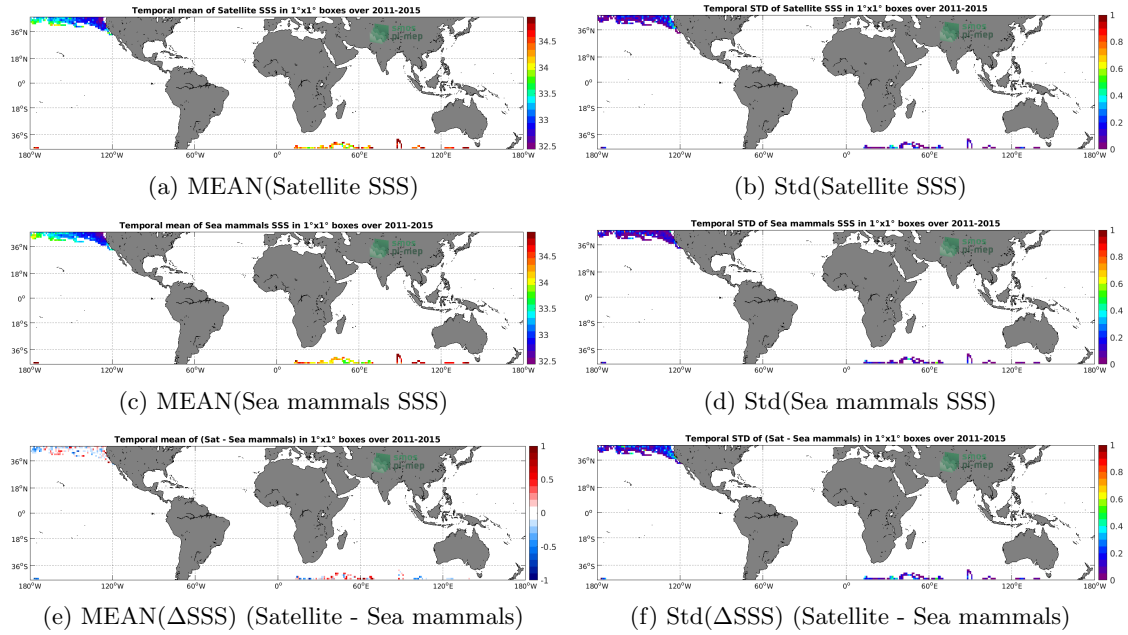
Figure 6: Temporal mean (left) and Std (right) of SSS from Aquarius SSS L3 OR v5 - 7-Day running (NASA-GSFC) (top), Sea mammals (middle), and of \Delta SSS (Satellite - Sea mammals). Only match-up pairs are used to generate these maps.
