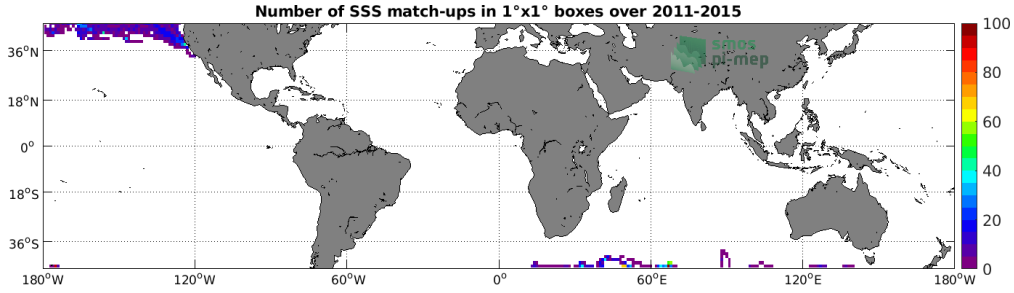
Figure 4: Number of SSS match-ups between Sea mammals SSS and the Aquarius SSS L3 OR v5 - 7-Day running (NASA-GSFC) SSS product for the Mid-Low Latitudes 45N-45S Pi-MEP region over 1^\circ \times 1^\circ boxes and for the full satellite product period.
