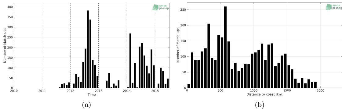
Figure 1: Number of match-ups between Sea mammals and Aquarius SSS L3 OR v5 - 7-Day running (NASA-GSFC) SSS as a function of time (a) and as function of the distance to coast (b) over the Mid-Low Latitudes 45N-45S Pi-MEP region and for the full satellite product period.
