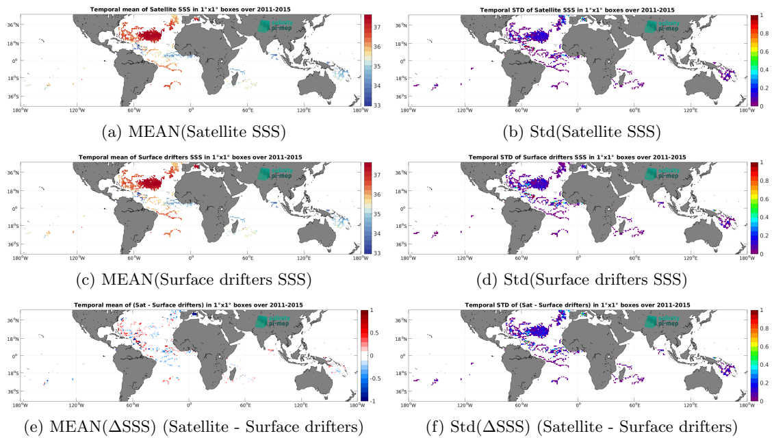
Figure 6: Temporal mean (left) and Std (right) of SSS from Aquarius SSS L3 OR v5 - 7-Day running (NASA-GSFC) (top), Surface drifters (middle), and of \Delta SSS (Satellite - Surface drifters). Only match-up pairs are used to generate these maps.
