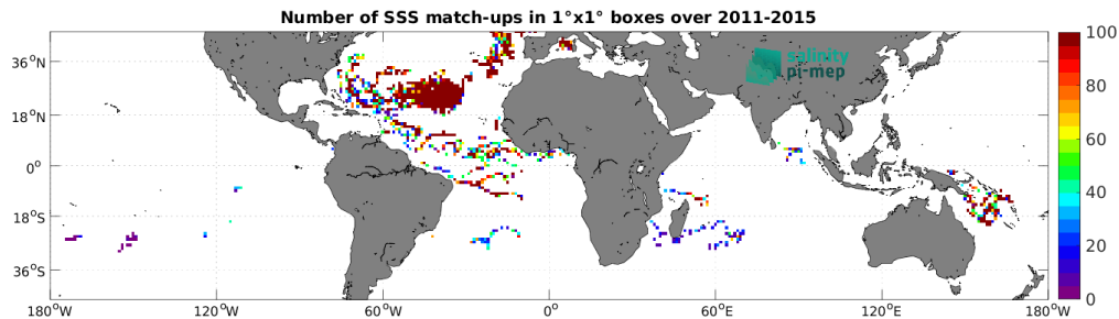
Figure 4: Number of SSS match-ups between Surface drifters SSS and the Aquarius SSS L3 OR v5 - 7-Day running (NASA-GSFC) SSS product for the Mid-Low Latitudes 45N-45S Pi-MEP region over 1^\circ \times 1^\circ boxes and for the full satellite product period.
