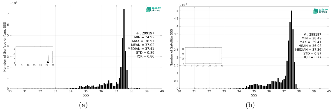
Figure 3: Histograms of SSS from Surface drifters (a) and Aquarius SSS L3 OR v5 - 7-Day running (NASA-GSFC) (b) considering all match-up pairs per bins of 0.1 over the Mid-Low Latitudes 45N-45S Pi-MEP region and for the full satellite product period.
