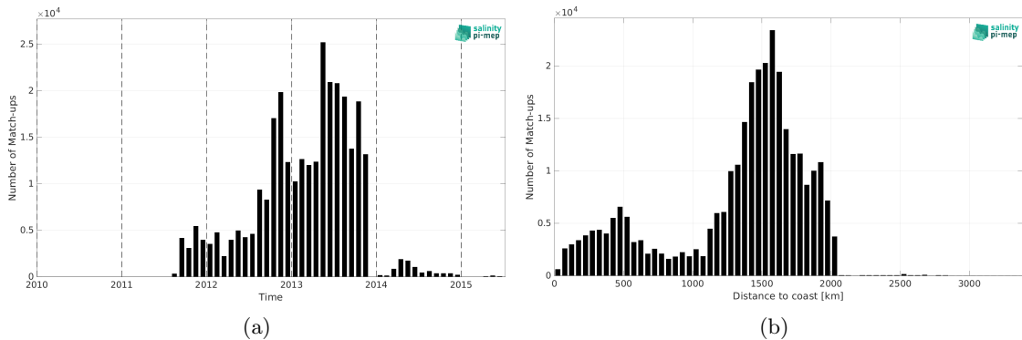
Figure 2: Number of match-ups between Surface drifters and Aquarius SSS L3 OR v5 - 7-Day running (NASA-GSFC) SSS as a function of time (a) and as function of the distance to coast (b) over the Mid-Low Latitudes 45N-45S Pi-MEP region and for the full satellite product period.
