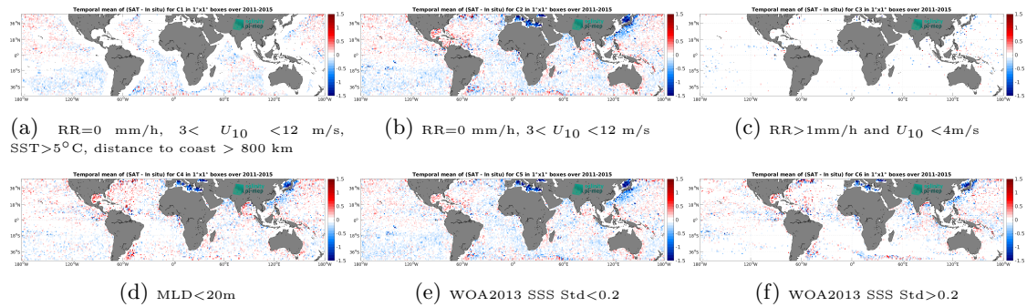
Figure 14: Temporal mean gridded over spatial boxes of size 1^\circ \times 1^\circ of \Delta\text{SSS} (Aquarius SSS L3 OR v5 - 7-Day running (NASA-GSFC) - Argo) for 6 different subdatasets corresponding to:RR=0 mm/h, 3 < U_{10} < 12 m/s, SST>5°C, distance to coast > 800 km (a), RR=0 mm/h, 3 < U_{10} < 12 m/s (b), RR>1mm/h and U_{10} < 4 m/s (c),MLD<20m (d),WOA2013 SSS Std<0.2 (e),WOA2013 SSS Std>0.2 (f).
