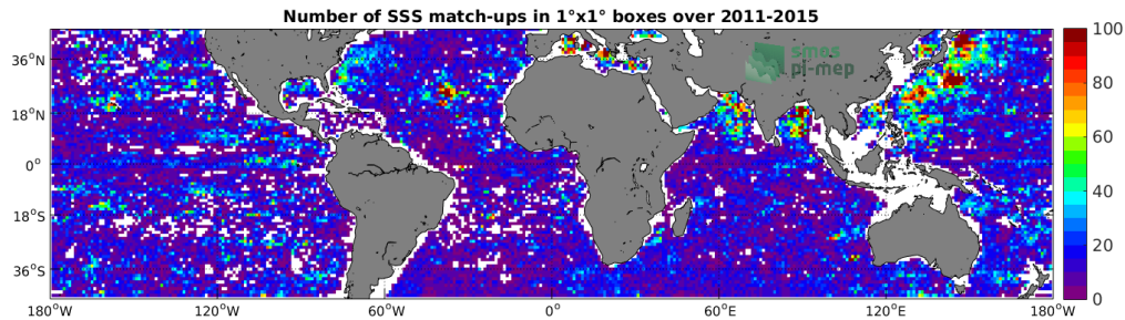
Figure 4: Number of SSS match-ups between Argo SSS and the Aquarius-L3-OR-V5-7DAY-RUNNING-1DEG SSS product for the Mid-Low Latitudes 45N-45S Pi-MEP region over 1^\circ \times 1^\circ boxes and for the full satellite product period.
