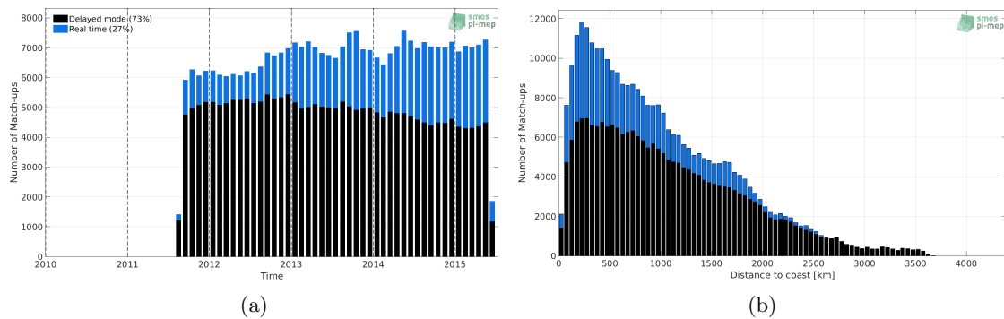
Figure 1: Number of match-ups between Argo and Aquarius-L3-OR-V5-7DAY-RUNNING-1DEG SSS as a function of time (a) and as function of the distance to coast (b) over the Mid-Low Latitudes 45N-45S Pi-MEP region and for the full satellite product period.
