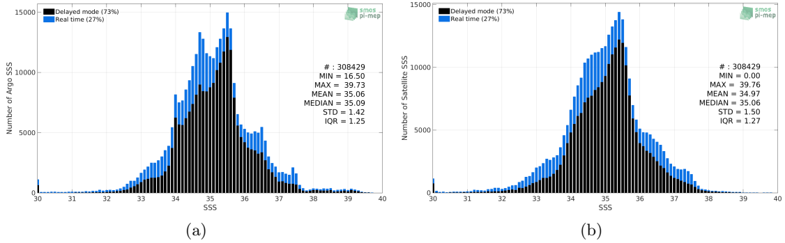
Figure 2: Histograms of SSS from Argos (a) and Aquarius-L3-OR-V5-7DAY-RUNNING-1DEG (b) considering all match-up pairs per bins of 0.1 over the Mid-Low Latitudes 45N-45S Pi-MEP region and for the full satellite product period.
