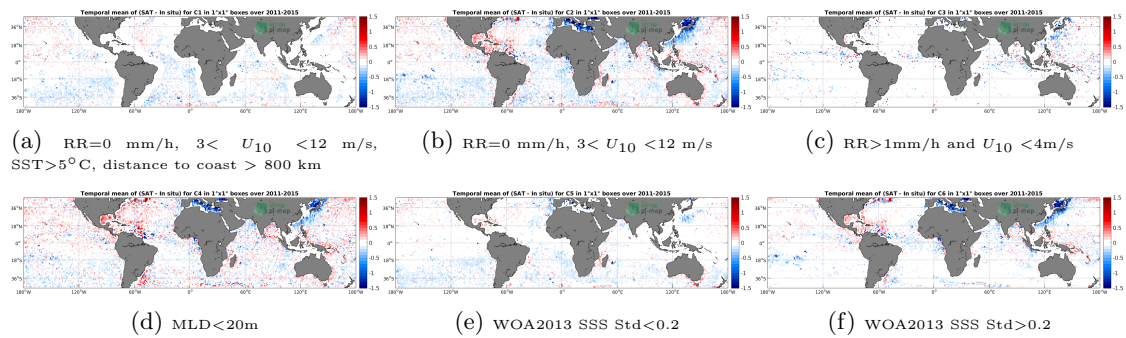
Figure 12: Temporal mean gridded over spatial boxes of size 1^\circ \times 1^\circ of \Delta SSS (Aquarius-L3-OR-V5-7DAY-RUNNING-1DEG - Argo) for 6 different subdatasets corresponding to:RR=0 mm/h, 3 < U_{10} < 12 m/s, SST >5^\circ C, distance to coast > 800 km (a), RR=0 mm/h, 3 < U_{10} < 12 m/s (b), RR >1 mm/h and U_{10} < 4 m/s (c),MLD <20 m (d),WOA2013 SSS Std <0.2 (e),WOA2013 SSS Std >0.2 (f).
