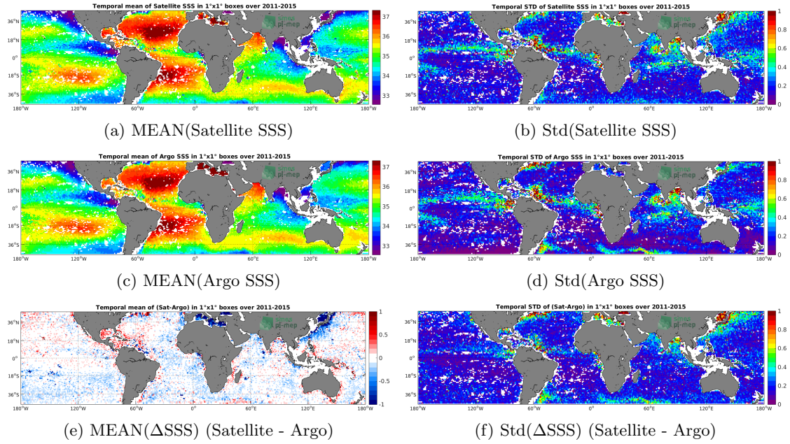
Figure 6: Temporal mean (left) and Std (right) of SSS from Aquarius-L3-OR-V5-7DAY-RUNNING-1DEG (top), Argo (middle), and of \Delta SSS (Satellite - Argo). Only match-up pairs are used to generate these maps.
